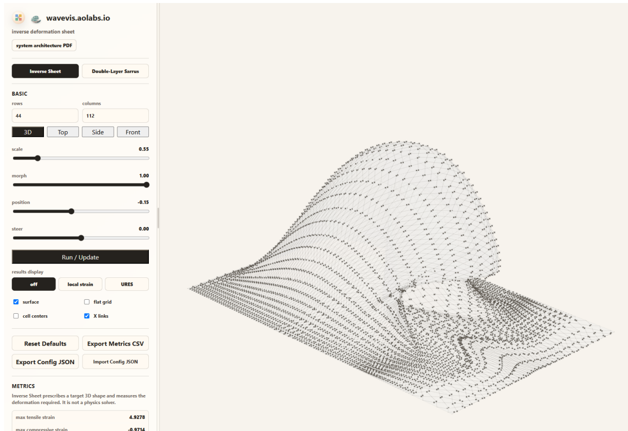
Figure 8. Candidate579 browser-rendered 3D/isometric view for the same default state. The default presentation retains the recovered geometry floor, restored isometric camera, source-profile readable surface skin, lighter isometric surface, pale wire grid, bounded 3D face-pinch transform, one-center four-leg X cells, physical connector pins, and a visible instanced shared-joint rod pass. Surface-on 3D preserves depth testing for hidden X/joint marks against the readable surface, reducing the false see-through throat wall without adding a fake bridge. This figure remains an improved open visual-match boundary rather than an exact reference match because the lip is still blunter and more capped than the June 24 tube reference.
