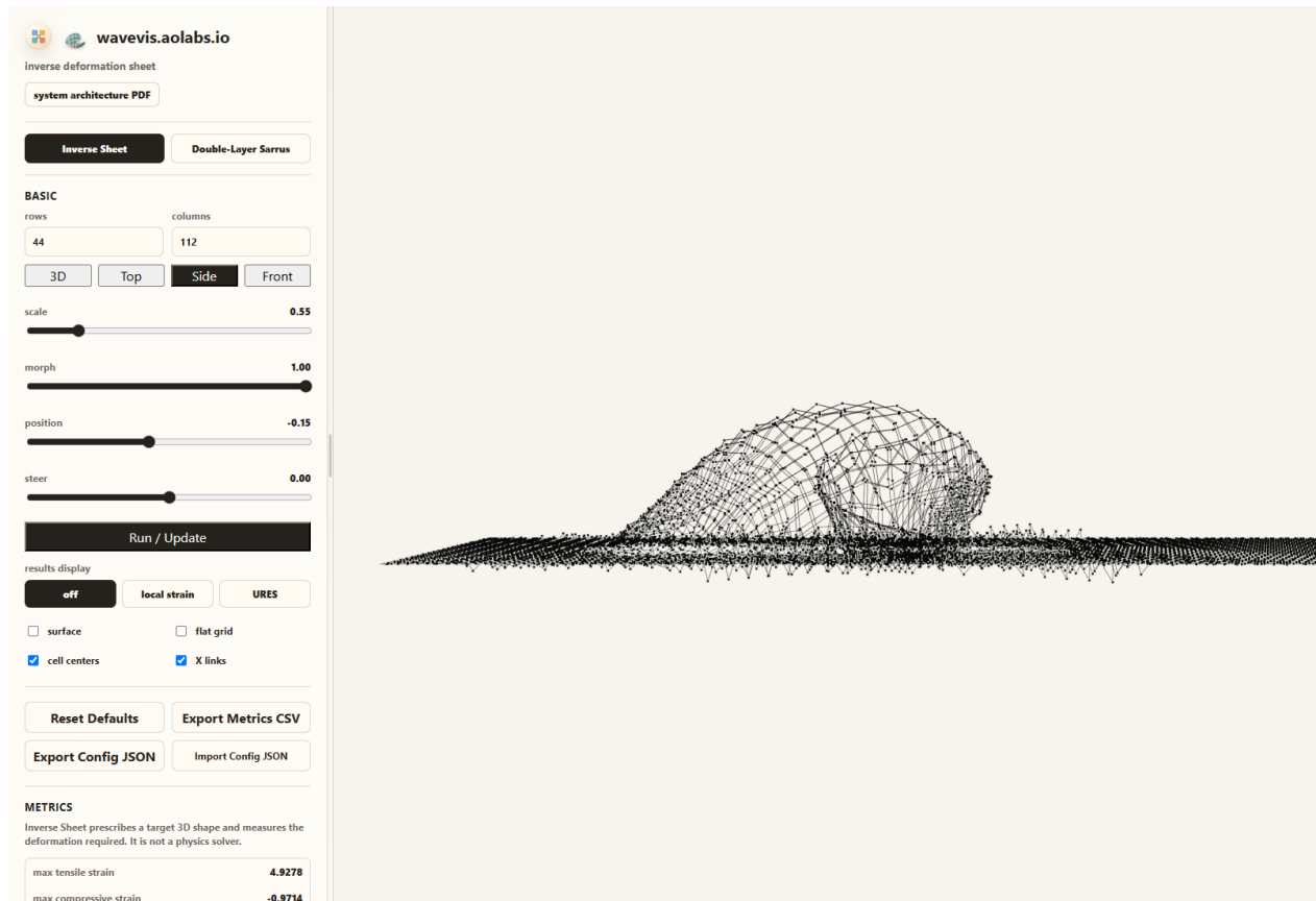
Figure 7. Candidate579 Side view with surface=0&connectors=1. This X-only evidence removes the surface skin and shows the actual mechanism layer: each cell is one center pivot with four center-to-connector legs; two legs form the sw-ne bar and two legs form the se-nw bar. Each bar is straight and bisected at the center pivot, the two bars may have different lengths, and neighboring cells meet at visible connector pins. Every physical connector is used by exactly two cells, not four.
