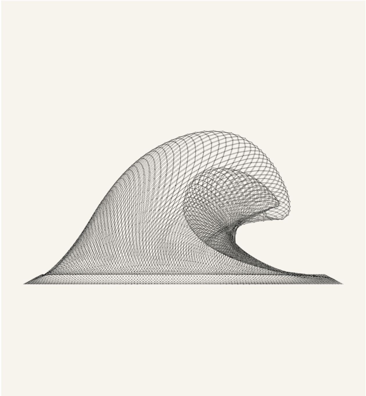
Figure 6. Candidate451 Side view with surface=0&connectors=1 . This X-only evidence removes the surface skin and shows the actual mechanism layer: each cell is a straight two-bar X, each diagonal is bisected at the center pivot, and neighboring cells meet at visible shared connector joints through real center-to-connector arms.
