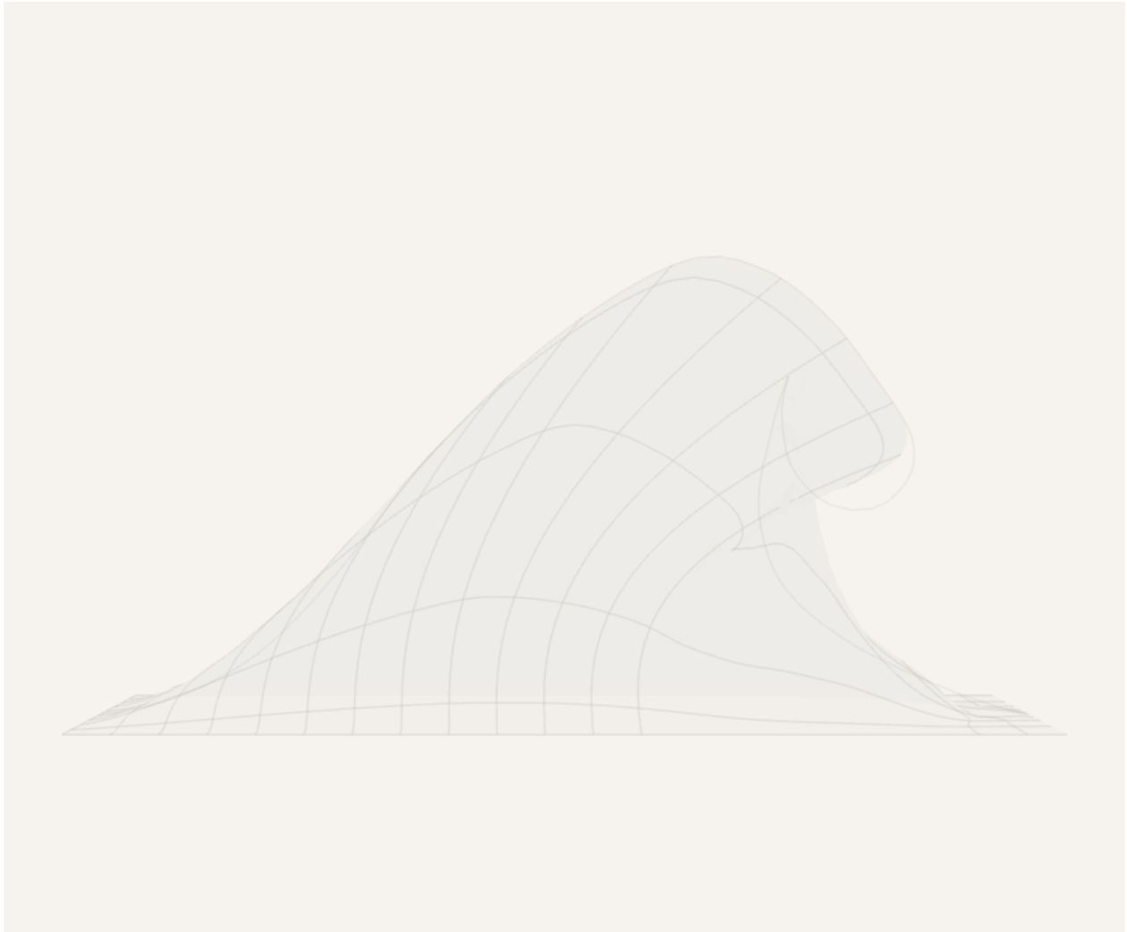
Figure 5. Candidate335 browser-rendered Side view for the default inverse-sheet state. The view is a full three-dimensional side camera with the smooth gridded sheet visible by default, not a cross-section. It retains the candidate330 side/lip state while the top plan repair stays isolated to Top view, preserving the open exact-match boundary.
