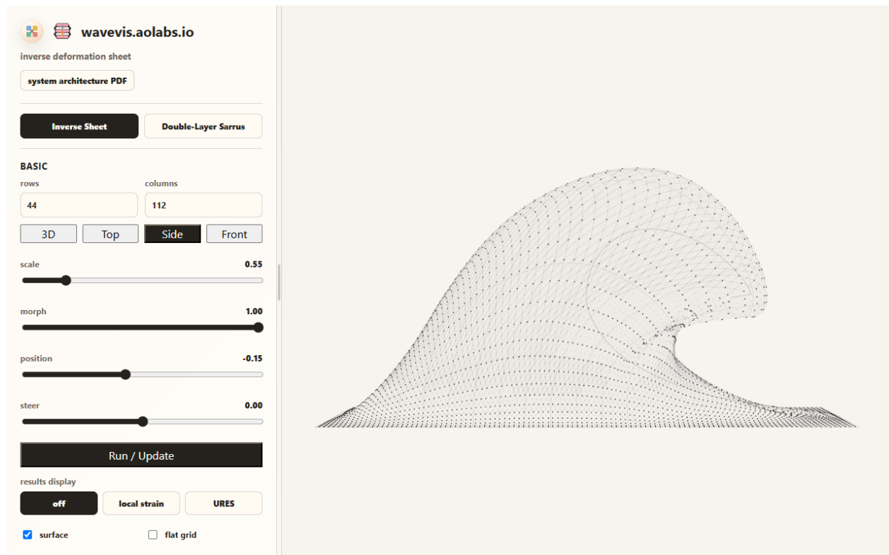
Figure 5. Candidate410 browser-rendered Side view for the default inverse-sheet state. The view is a full three-dimensional side camera with the readable surface, straight X-cell diagonals, center pivots, and shared connector joints visible together. It preserves the open exact-match boundary: the underside is more readable than the rejected skirt branch, but the reference-wave match is still not closed.
