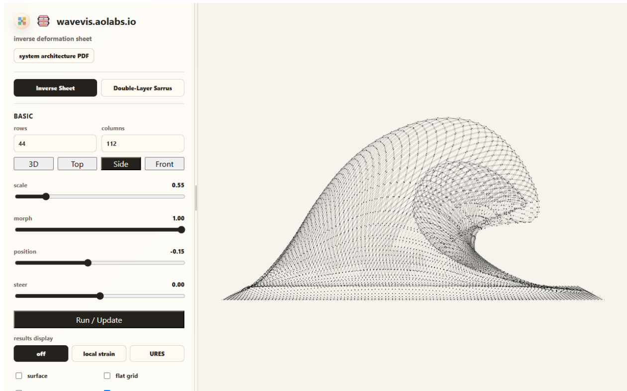
Figure 6. Candidate410 Side view with surface=0&connectors=1 . This X-only evidence removes the surface skin and shows the actual mechanism layer: each cell is a straight two-bar X, each diagonal is bisected at the center pivot, and neighboring cells meet at visible shared connector joints.
