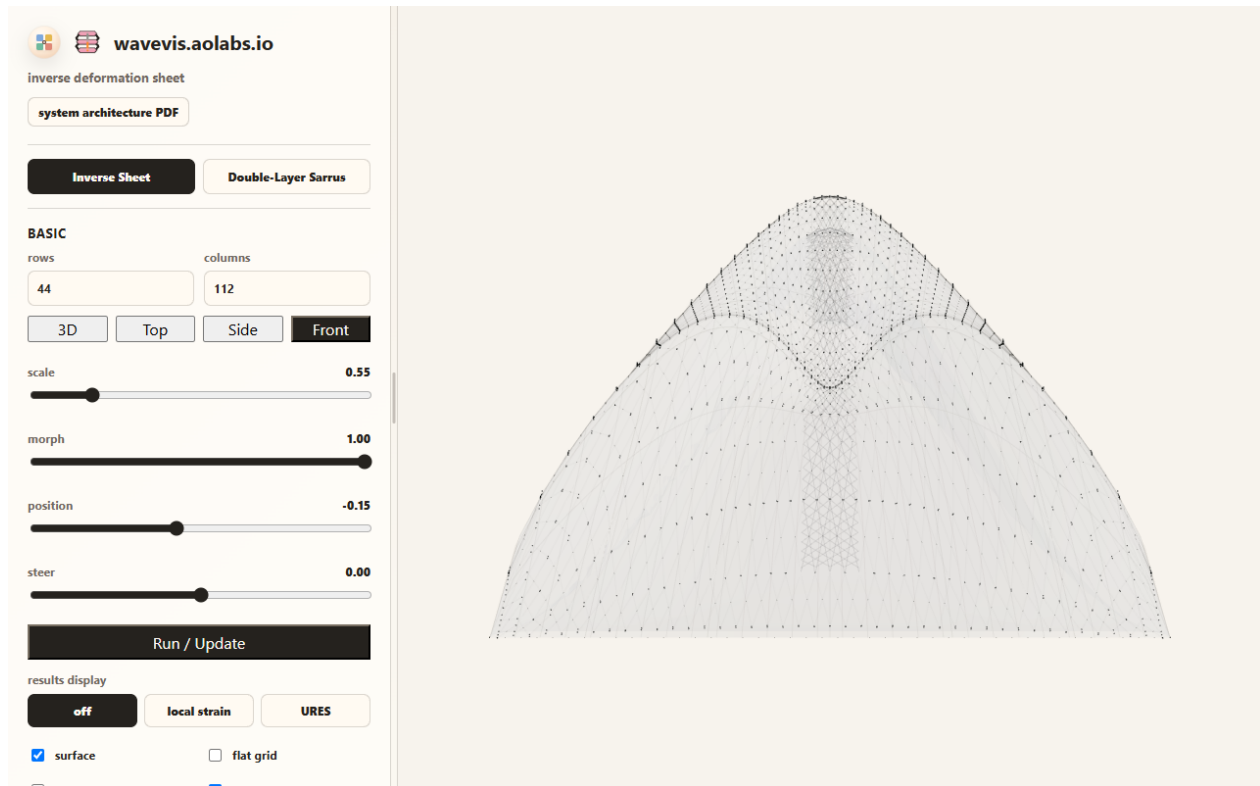
Figure 8. Candidate410 browser-rendered Front view for the same default state. This separate product camera compresses front depth, bounds the terminal lip contribution, depth-tests the pale grid against the lip, keeps rounded terminal width, and shows the center X-cell linkage through the projected cap rather than hiding mechanism state behind a pasted cap layer. The June 27 projection checkpoint remains open against the June 24 front reference.
