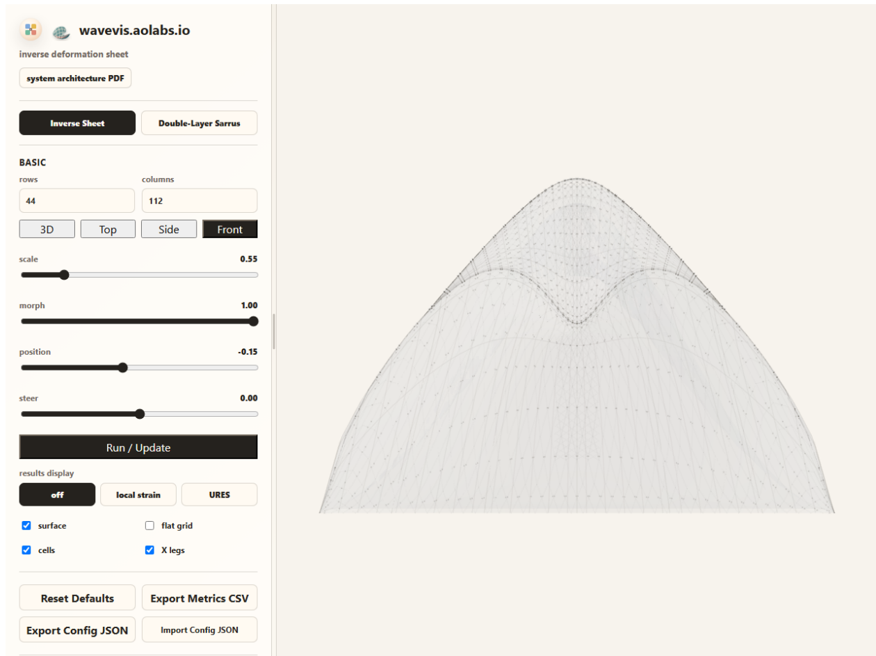
Figure 9. Candidate620 browser-rendered Front view retained as the separate spanwise product camera. This view compresses front depth, bounds the terminal lip contribution, depth-tests the pale grid against the lip, keeps rounded terminal width, and shows the black-square X-cell linkage with spherical connector nodes through the projected cap rather than hiding mechanism state behind a pasted cap layer. The projection checkpoint remains open against the June 24 and June 28 references.
