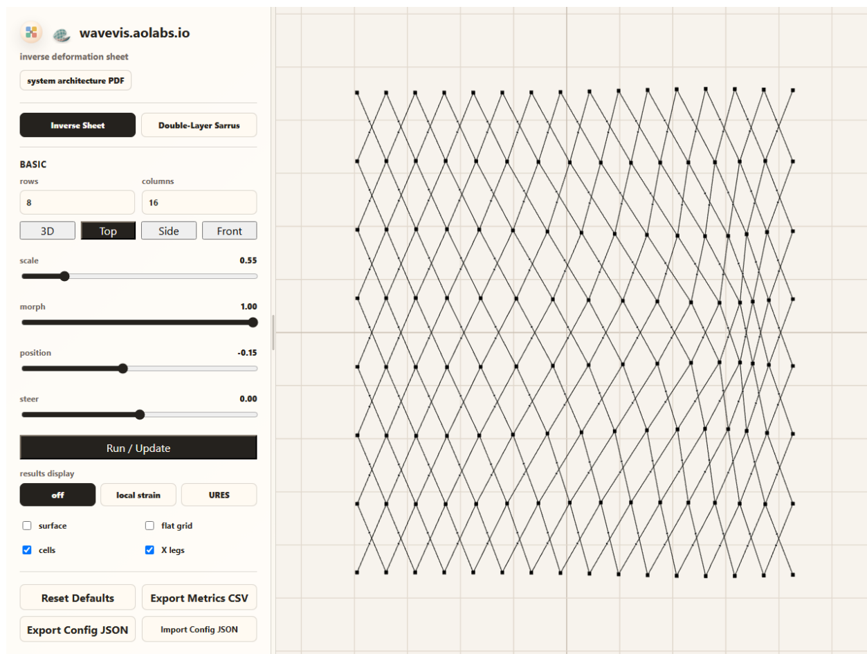
Figure 13. Candidate620 inspectable Top proof with rows=8, columns=16, surface=0, connectors=1, and cells=1. This low-density route exists so the hard cell contract can be inspected directly through the X legs and cells layers: a cell is not two nearby two-leg elements; it is one black square with four straight legs, and each visible connector is a spherical center-pair node used by exactly two neighboring cells.
