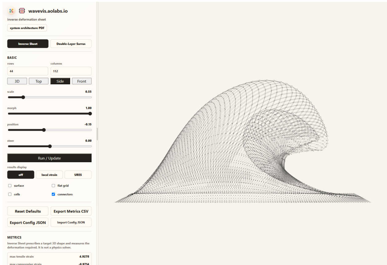
Figure 6. Candidate426 Side view with surface=0&connectors=1. This X-only evidence removes the surface skin and shows the actual mechanism layer: each cell is a straight two-bar X, each diagonal is bisected at the center pivot, and neighboring cells meet at visible shared connector joints.
