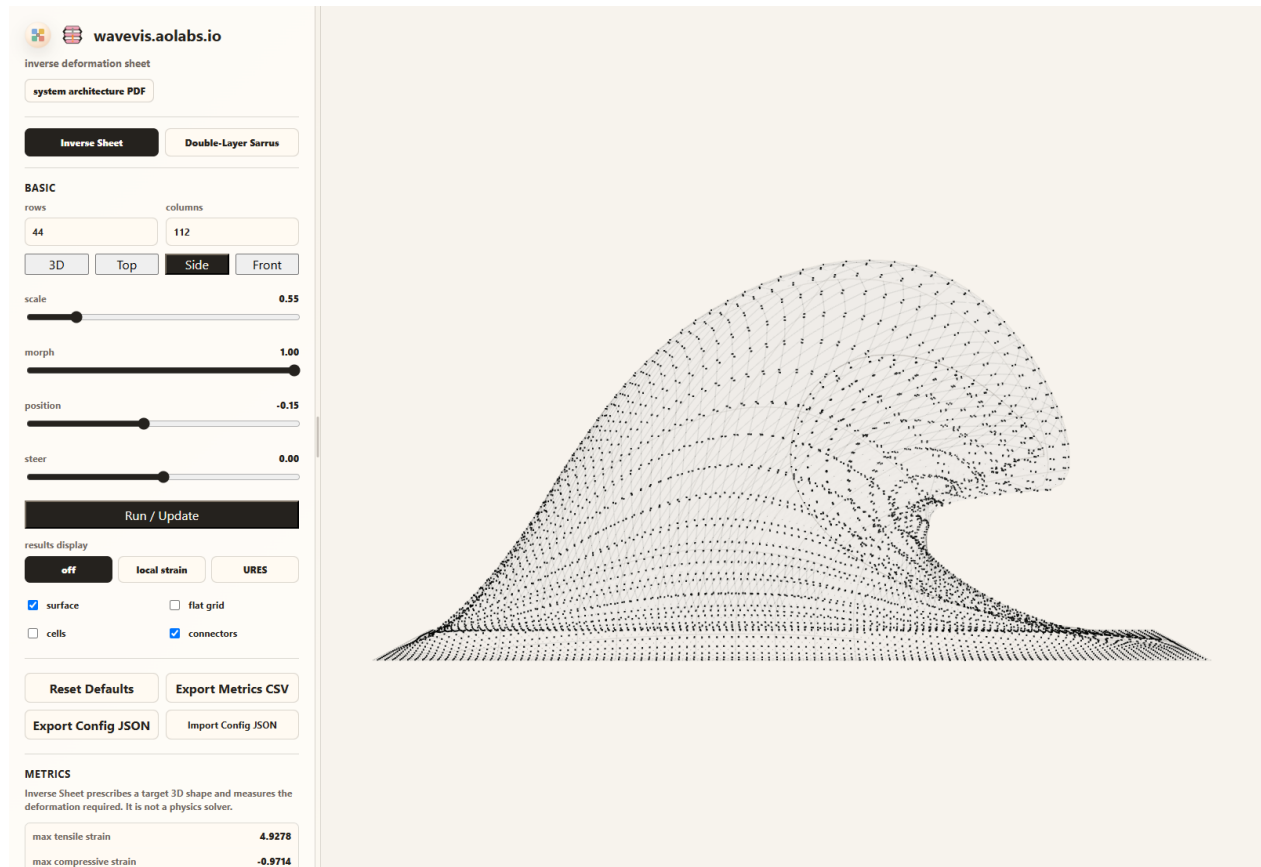
Figure 5. Candidate426 browser-rendered Side view for the default inverse-sheet state. The view is a full three-dimensional side camera with the readable surface, straight X-cell diagonals, center pivots, and enlarged shared connector joints visible together. It preserves the open exact-match boundary: the underside is more readable than the rejected skirt branch, but the reference-wave match is still not closed.
