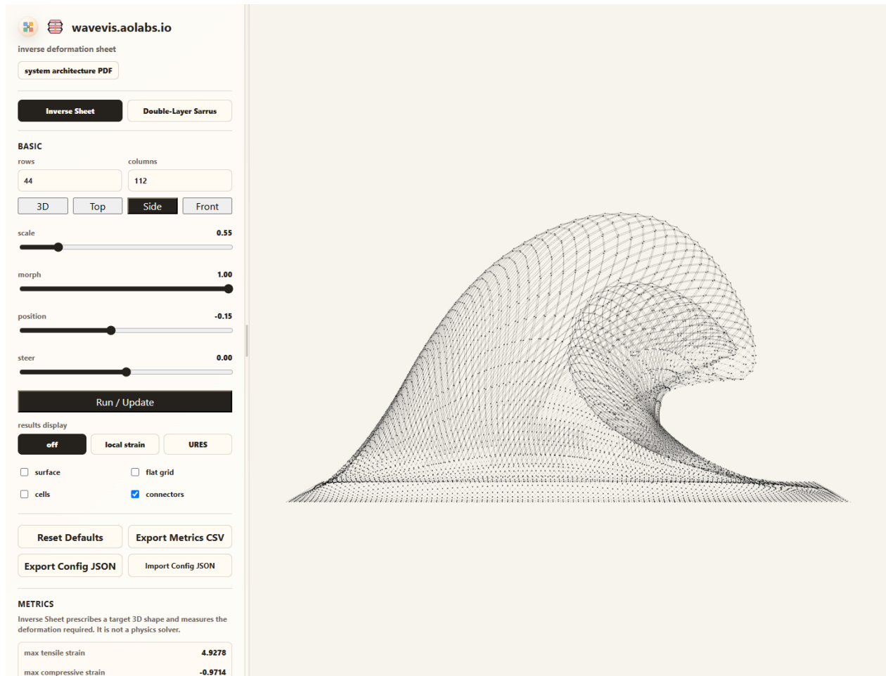
Figure 6. Candidate412 Side view with surface=0&connectors=1. This X-only evidence removes the surface skin and shows the actual mechanism layer: each cell is a straight two-bar X, each diagonal is bisected at the center pivot, and neighboring cells meet at visible shared connector joints.
