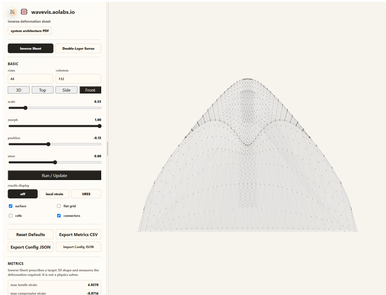
Figure 8. Candidate412 browser-rendered Front view for the same default state. This separate product camera compresses front depth, bounds the terminal lip contribution, depth-tests the pale grid against the lip, keeps rounded terminal width, and shows the center X-cell linkage through the projected cap rather than hiding mechanism state behind a pasted cap layer. The June 27 projection checkpoint remains open against the June 24 front reference.
