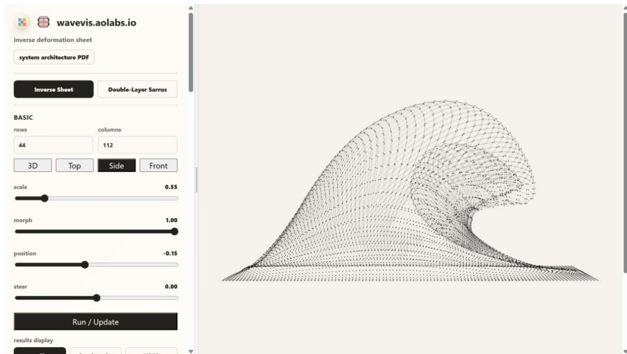
Figure 6. Candidate406 Side view with surface=0&connectors=1 . This X-only evidence removes the surface skin and shows the actual mechanism layer: each cell is a straight two-bar X, each diagonal is bisected at the center pivot, and neighboring cells meet at visible shared connector joints.
