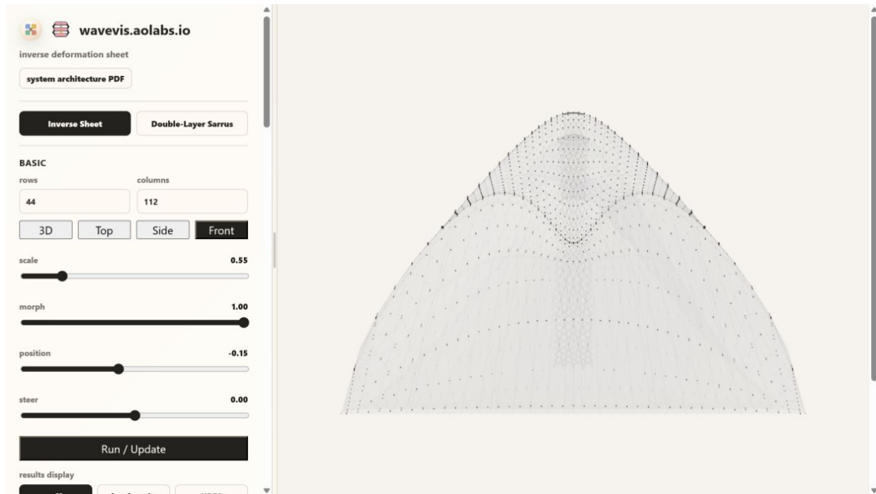
Figure 8. Candidate406 browser-rendered Front view for the same default state. This separate product camera compresses front depth, bounds the terminal lip contribution, depth-tests the pale grid against the lip, keeps rounded terminal width, and shows the center X-cell linkage through the projected cap rather than hiding mechanism state behind a pasted cap layer. The June 27 projection checkpoint remains open against the June 24 front reference.
