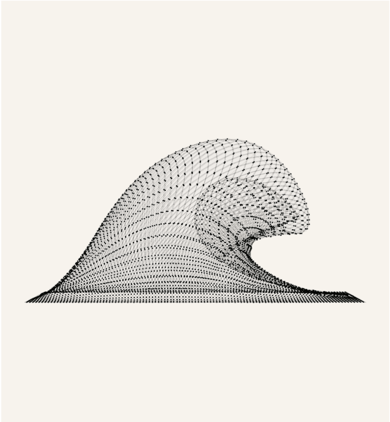
Figure 5. Candidate464 browser-rendered Side view for the default inverse-sheet state. The view is a full three-dimensional side camera with the readable surface, straight X-cell diagonals, center pivots, shared connector joints, and shared-joint arms visible together. It preserves the open exact-match boundary: the underside remains readable and the between-cell joints are clearer, but the reference-wave match is still not closed.
