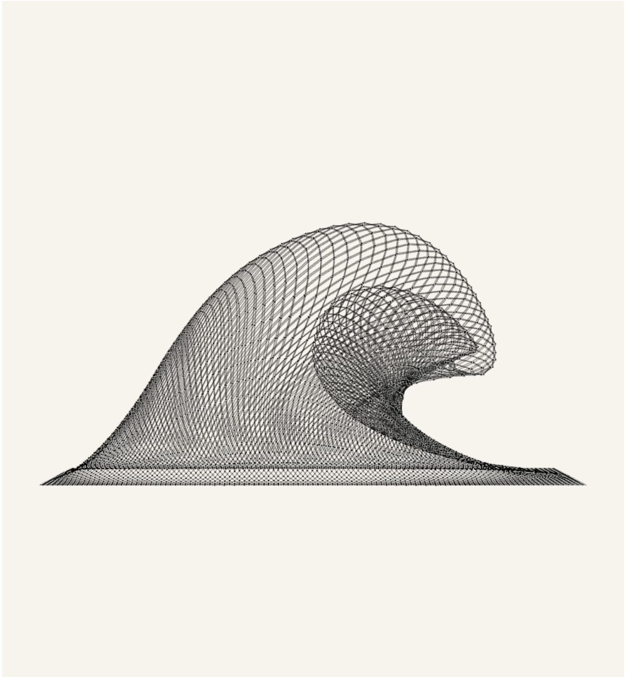
Figure 6. Candidate464 Side view with surface=0&connectors=1 . This X-only evidence removes the surface skin and shows the actual mechanism layer: each cell is a straight two-bar X, each diagonal is bisected at the center pivot, and neighboring cells meet at visible shared connector joints through real center-to-connector arms.
