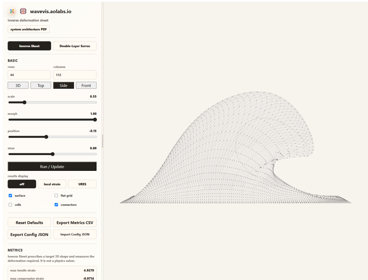
Figure 5. Candidate413 browser-rendered Side view for the default inverse-sheet state. The view is a full three-dimensional side camera with the readable surface, straight X-cell diagonals, center pivots, and shared connector joints visible together. It preserves the open exact-match boundary: the underside is more readable than the rejected skirt branch, but the reference-wave match is still not closed.
