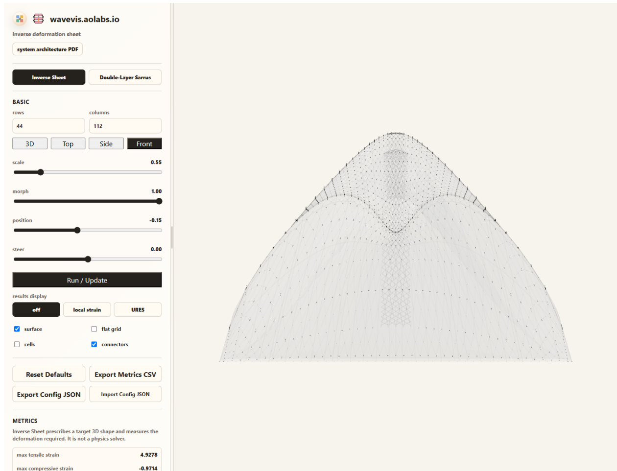
Figure 8. Candidate413 browser-rendered Front view for the same default state. This separate product camera compresses front depth, bounds the terminal lip contribution, depth-tests the pale grid against the lip, keeps rounded terminal width, and shows the center X-cell linkage through the projected cap rather than hiding mechanism state behind a pasted cap layer. The June 27 projection checkpoint remains open against the June 24 front reference.
