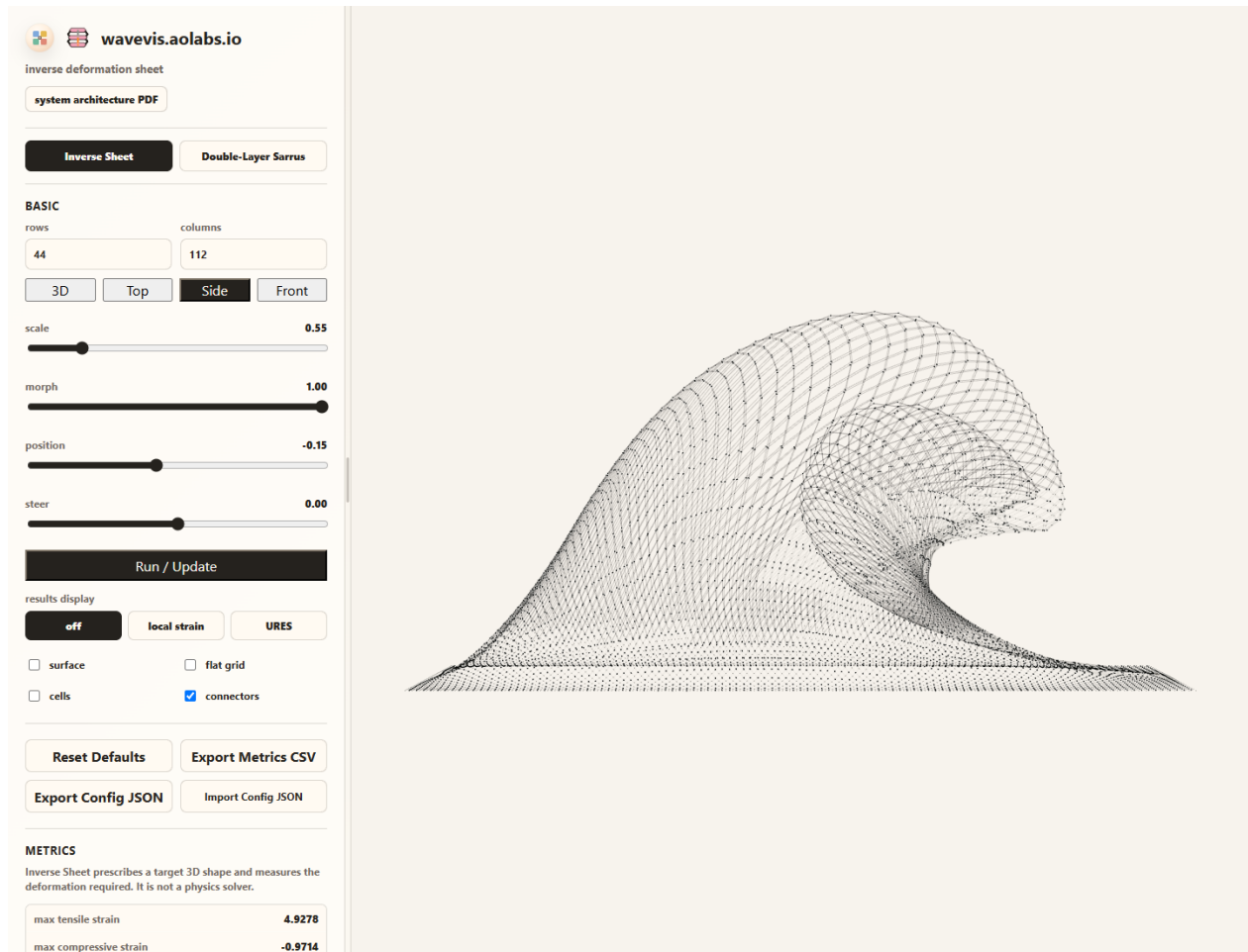
Figure 6. Candidate413 Side view with surface=0&connectors=1. This X-only evidence removes the surface skin and shows the actual mechanism layer: each cell is a straight two-bar X, each diagonal is bisected at the center pivot, and neighboring cells meet at visible shared connector joints.
