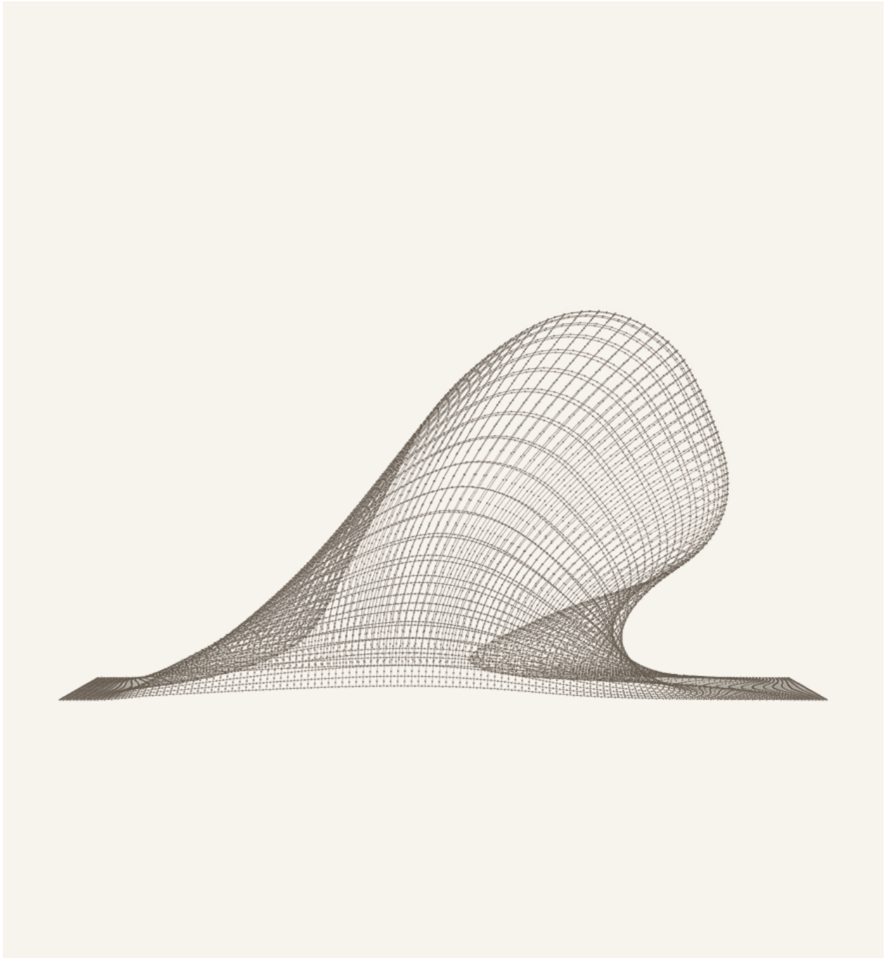
Figure 6. Candidate738 browser-rendered Side view for the default inverse-sheet state. The view keeps the readable surface subordinate to the actual mechanism: a lighter surface skin, muted X-cell ink, one-center/four-leg cell bodies, spherical two-use connector nodes, and visible shared-joint rods remain readable without forming a black silhouette mass. Candidate738 opens the inner throat, starts side/isometric terminal narrowing earlier, and lightens the side mechanism ink so the full sheet remains visible instead of reading as either a surface shell, a black silhouette, or a hard angular knot. The underside no longer contains the rejected bowl/dimple/cavity family, the perimeter border band is source-gated to stay flat, and Side uses a view-specific smoothed curled profile rather than the capped Candidate661 side path. The reference-wave match is still open: this checkpoint repairs the surface-silhouette failure and reduces the angular throat read, but it remains sparse and approximate rather than a completed Moana-like plunge.
