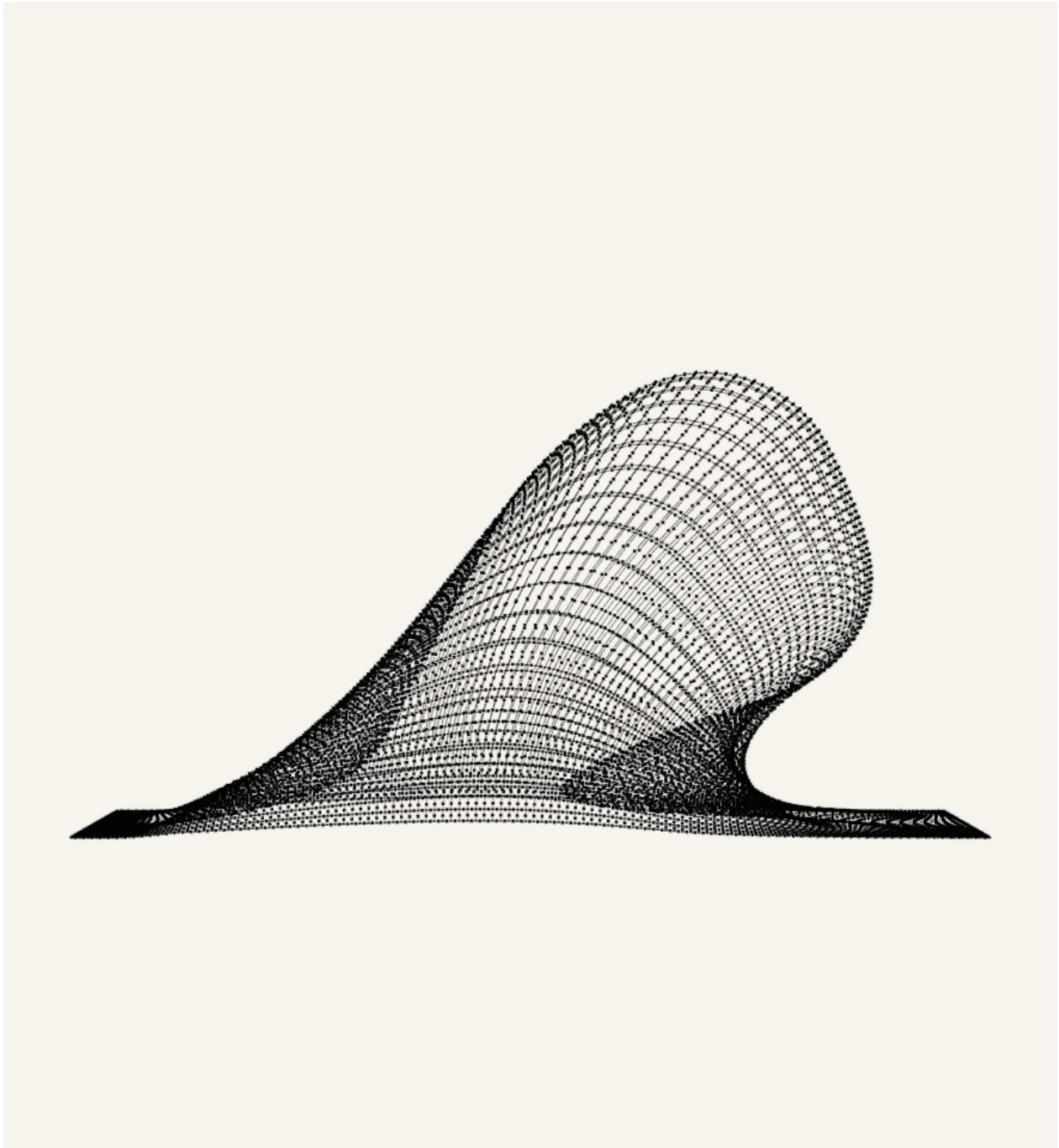
Figure 7. Candidate738 Side view with surface=0&connectors=1&cells=1 . This X-only evidence removes the surface skin and shows the actual mechanism layer after the side readable-profile split: each cell is one black square with four straight center-to-connector legs, opposite pairs are equal length and collinear through the cell center, and every connector is a spherical physical node with exactly two attached leg uses. Neighboring cells meet through visible connector nodes; no between-cell connector is allowed to become an X or a four-cell joint.
