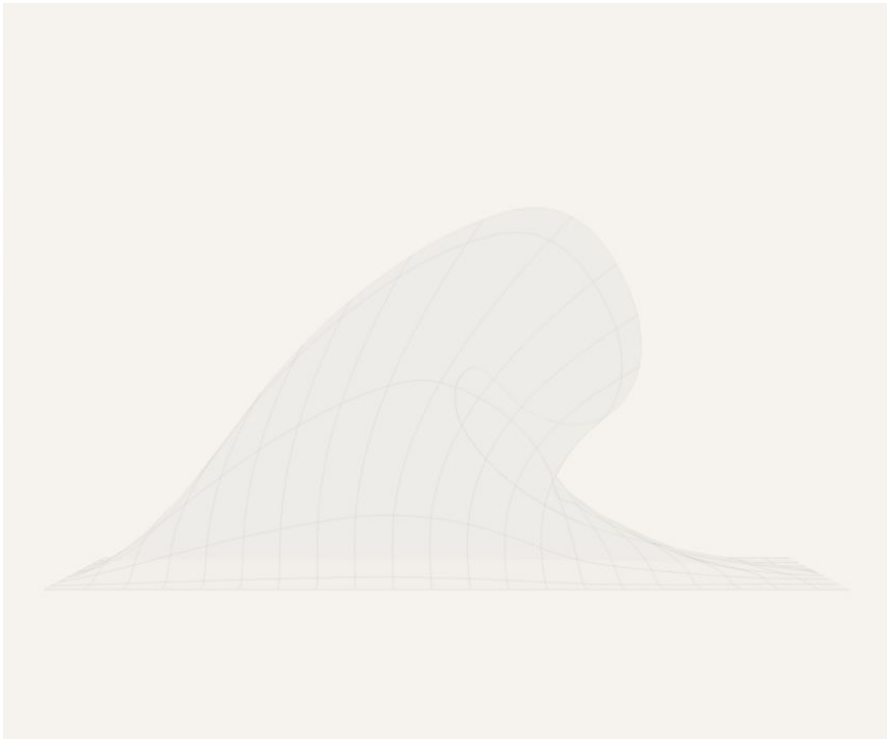
Figure 5. Current source-rendered Side view for the default inverse-sheet state. The view is a full three-dimensional side camera with the smooth gridded sheet visible by default, not a cross-section. It uses the compact forward/downturned source curl profile to keep the open-throat attempt, curled lip, downturned tip, and overhang visible with pale depth-written side skin and thinned guide rows, while preserving the open exact-match boundary.
