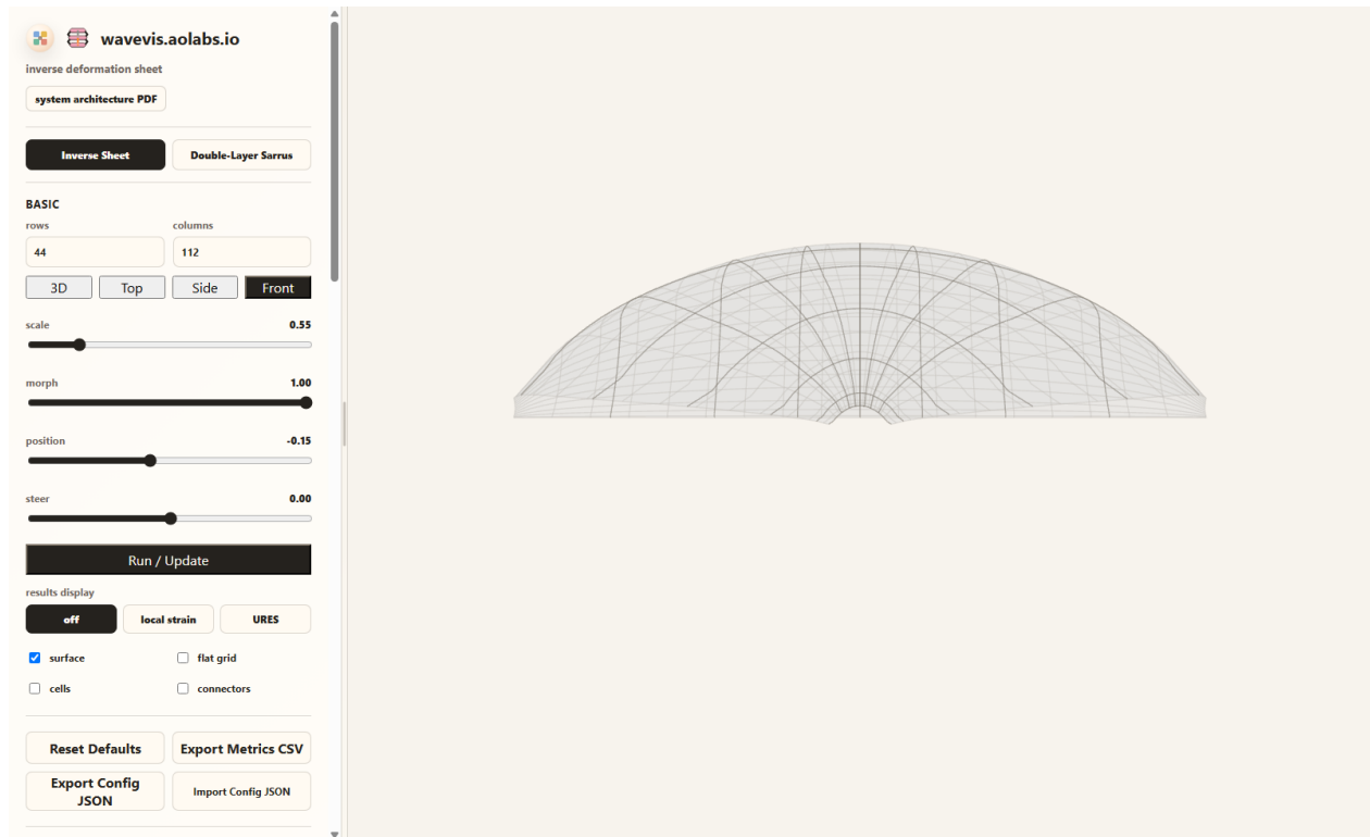
Figure 5. Current source-rendered Front view for the same default state. This view was added as a separate product camera so the spanwise mound and lip-cap read can be checked directly against the June 24 three-view reference.
