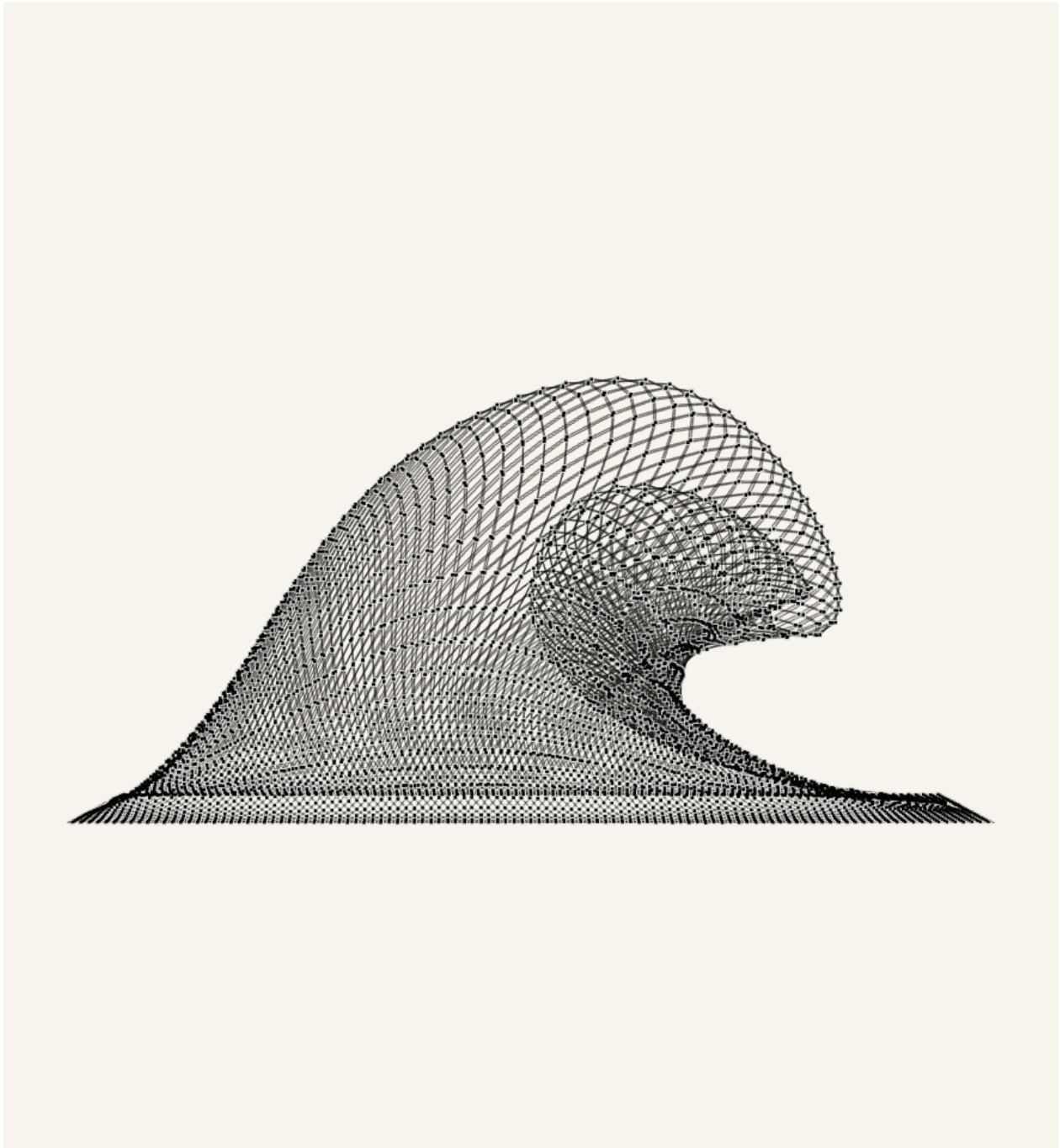
Figure 6. Candidate529 Side view with surface=0&connectors=1 . This X-only evidence removes the surface skin and shows the actual mechanism layer: each cell is a straight two-bar X, each diagonal is bisected at the center pivot, and neighboring cells meet at visible shared connector pins through real center-to-connector rods.
