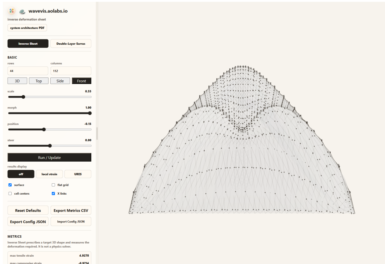
Figure 9. Candidate579 browser-rendered Front view retained as the separate spanwise product camera. Candidate611 did not alter the front solver path. This view compresses front depth, bounds the terminal lip contribution, depth-tests the pale grid against the lip, keeps rounded terminal width, and shows the one-center X-cell linkage through the projected cap rather than hiding mechanism state behind a pasted cap layer. The projection checkpoint remains open against the June 24 and June 28 references.
