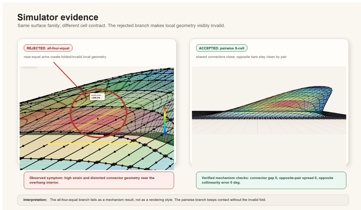
Figure 16. Simulator evidence for the linkage direction. The current architecture must keep this mechanism truth visible while the inverse target shape is improved.
