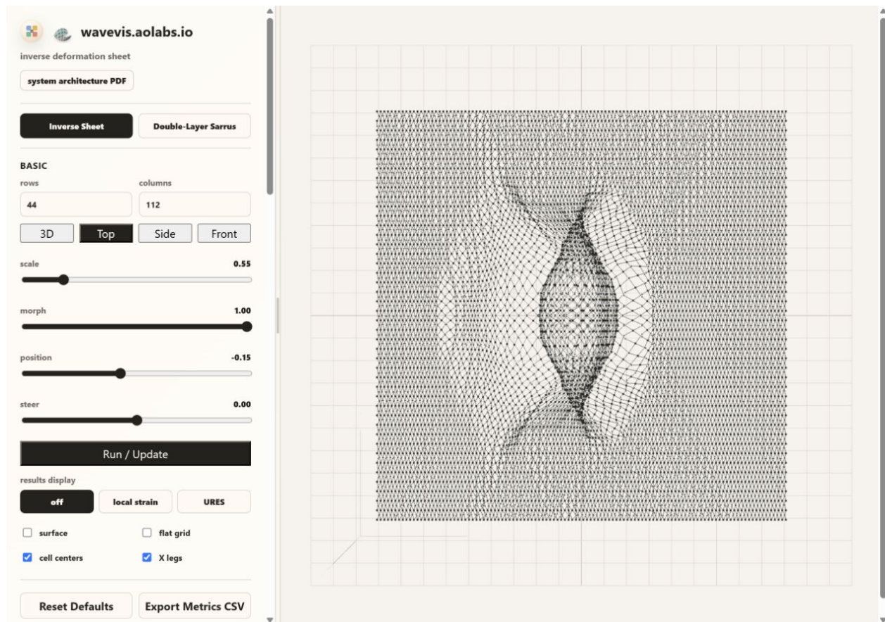
Figure 12. Candidate611 Top view with surface=0&connectors=1&cells=1. This proof view is intentionally dense because it shows the whole array. Each visible cell center is the pivot for four straight legs; opposite leg pairs form the two bisected X bars, and adjacent cells meet at two-cell connector pins. This is the current hard mechanism acceptance test, not a decorative overlay.
