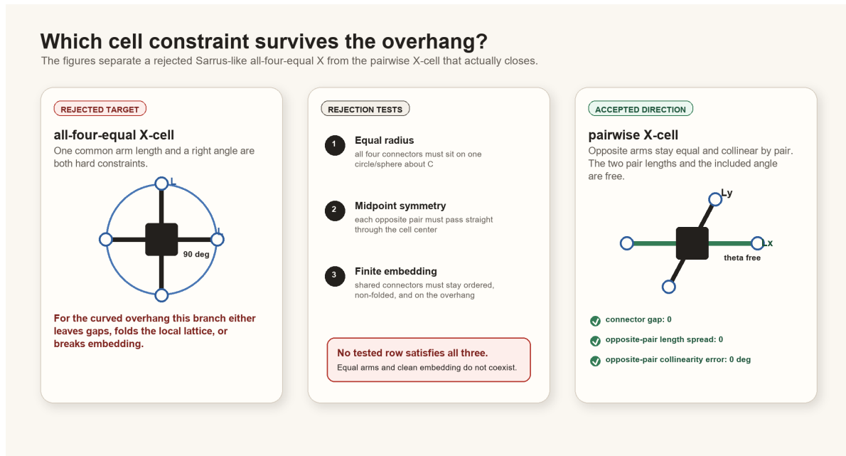
Figure 15. Mechanism contract inherited from the constraint proof and updated in the current renderer. WaveVis should preserve exact shared contact, straight X bars, and pairwise equal, collinear opposite halves rather than hiding infeasible all-four-equal geometry behind filler surfaces.
