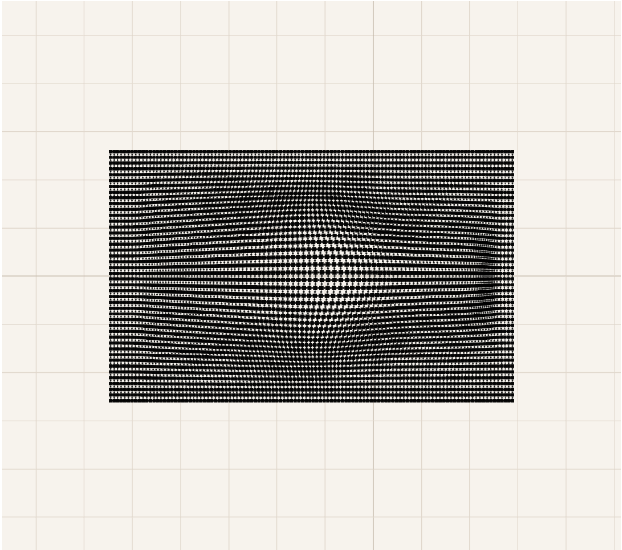
Figure 12. Candidate714 Top view with surface=0&connectors=1&cells=1 . This proof view is intentionally dense because it shows the whole array through the X legs and cells layers. Each visible black square cell is the body for four straight legs, each opposite pair remains collinear/equal through the center, and adjacent cells meet at spherical two-use connector nodes. This is the current hard mechanism acceptance test, not a decorative overlay.
