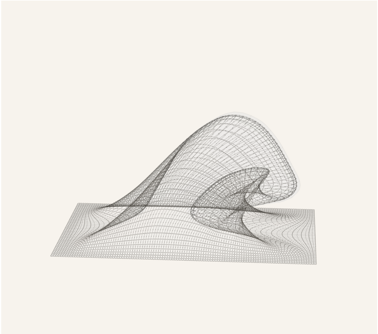
Figure 8. Candidate714 browser-rendered 3D/isometric view for the same default state. The default presentation retains the recovered geometry floor, a lower side-biased isometric camera, smoothed curled readable surface skin, pale wire grid, visible four-leg X cells, spherical two-use connector nodes, and grey mechanism ink tuned away from the rejected silhouette pass. The 3D view is still a mechanism view, not a surface-only substitute. This figure remains an improved open visual-match boundary rather than an exact reference match.
