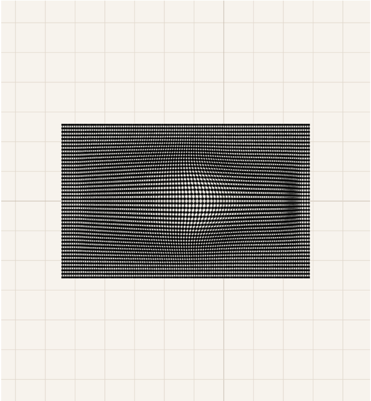
Figure 12. Candidate696 Top view with surface=0&connectors=1&cells=1 . This proof view is intentionally dense because it shows the whole array through the X legs and cells layers. Each visible black square cell is the body for four straight legs, each opposite pair remains collinear/equal through the center, and adjacent cells meet at spherical two-use connector nodes. This is the current hard mechanism acceptance test, not a decorative overlay.
