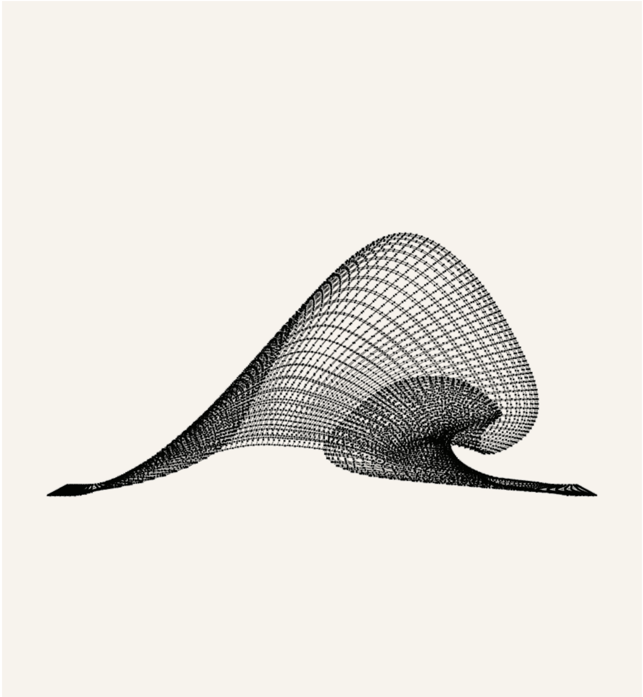
Figure 7. Candidate696 Side view with surface=0&connectors=1&cells=1 . This X-only evidence removes the surface skin and shows the actual mechanism layer after the side readable-profile split: each cell is one black square with four straight center-to-connector legs, opposite pairs are equal length and collinear through the cell center, and every connector is a spherical physical node with exactly two attached leg uses. Neighboring cells meet through visible connector nodes; no between-cell connector is allowed to become an X or a four-cell joint.
