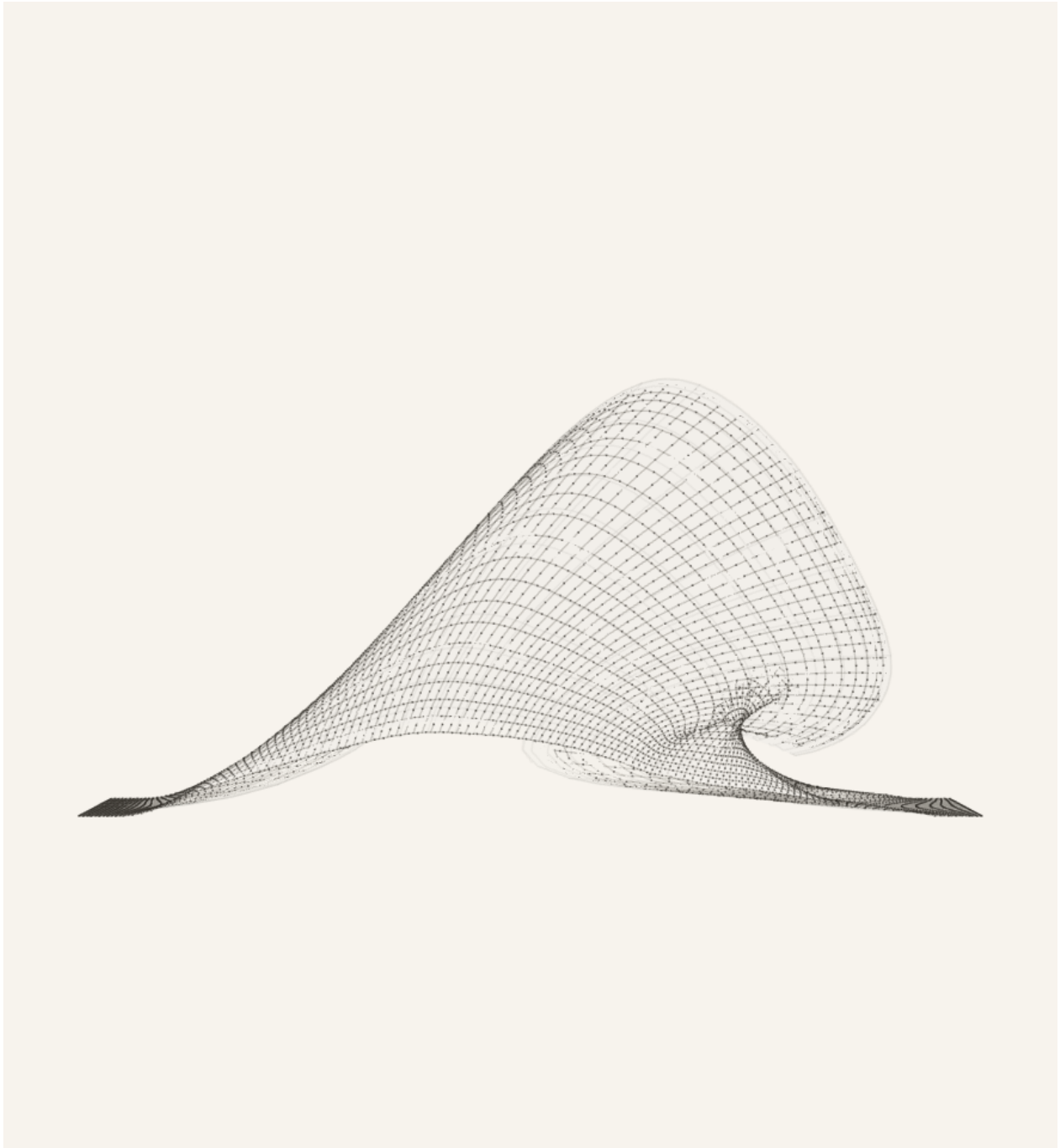
Figure 6. Candidate696 browser-rendered Side view for the default inverse-sheet state. The view keeps the readable surface subordinate to the actual mechanism: lighter side wire grid, black square one-center/four-leg cells, spherical two-use connector nodes, and instanced shared-joint rods are visible together. The underside no longer contains the rejected bowl/dimple/cavity family, the perimeter border band is source-gated to stay flat, and Side uses a view-specific open-barrel readable profile rather than the capped Candidate661 side path. The reference-wave match is still open: this checkpoint now reads as an open barrel/curl, but it remains sparse and approximate rather than a completed Moana-like plunge.
