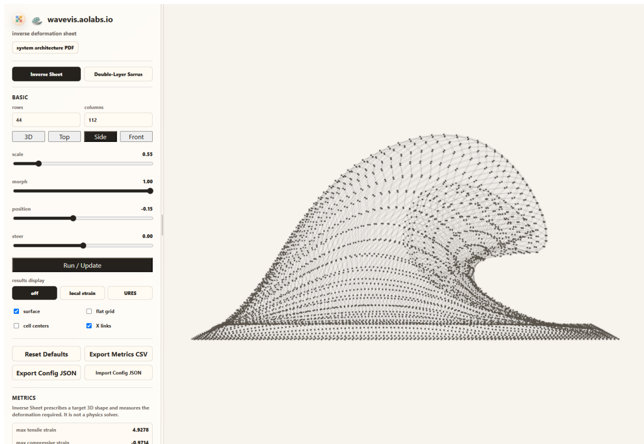
Figure 6. Candidate578 browser-rendered Side view for the default inverse-sheet state. The view is a full three-dimensional side camera with the readable surface, light side wire grid, straight X-cell diagonals, center pivots, physical shared connector pins, and instanced shared-joint rods visible together. It preserves the open exact-match boundary: the underside remains readable and the between-cell joints stay explicit, but the reference-wave match is still not closed.
