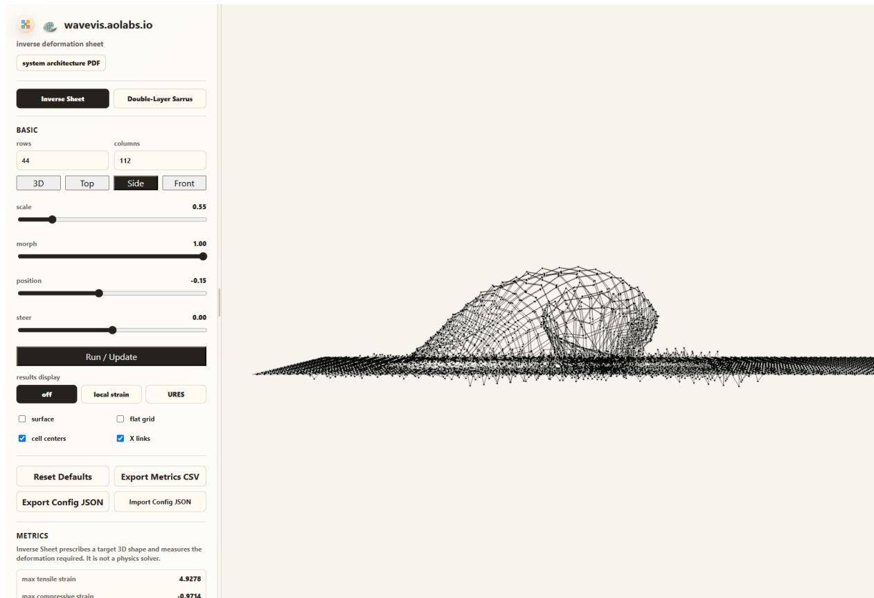
Figure 7. Candidate578 Side view with surface=0&connectors=1. This X-only evidence removes the surface skin and shows the actual mechanism layer: each cell is a straight two-bar X, each diagonal is bisected at the center pivot, and neighboring cells meet at visible connector pins through real center-to-connector rods. Every physical connector is used by exactly two cells, not four.
