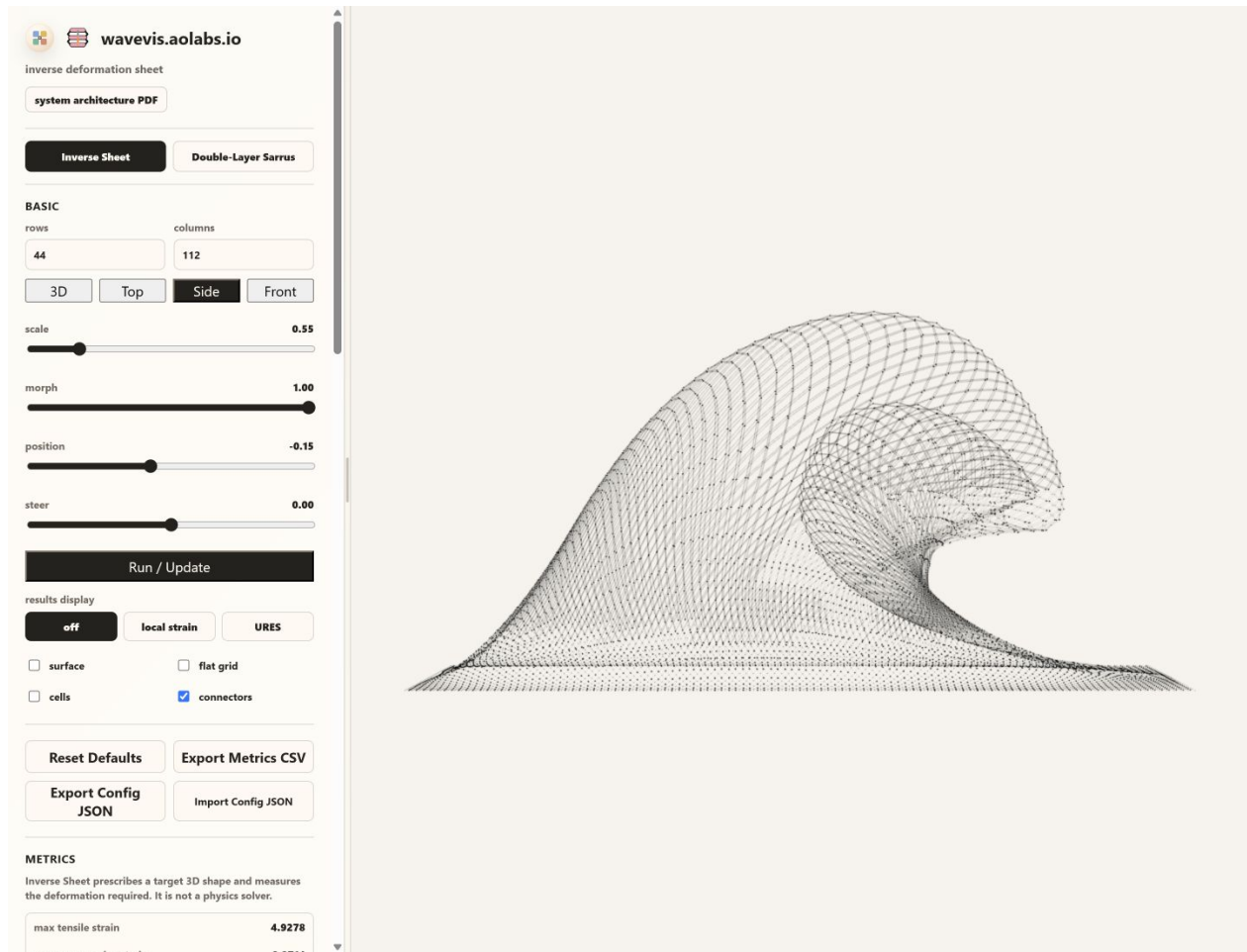
Figure 6. Candidate421 Side view with surface=0&connectors=1. This X-only evidence removes the surface skin and shows the actual mechanism layer: each cell is a straight two-bar X, each diagonal is bisected at the center pivot, and neighboring cells meet at visible shared connector joints.
