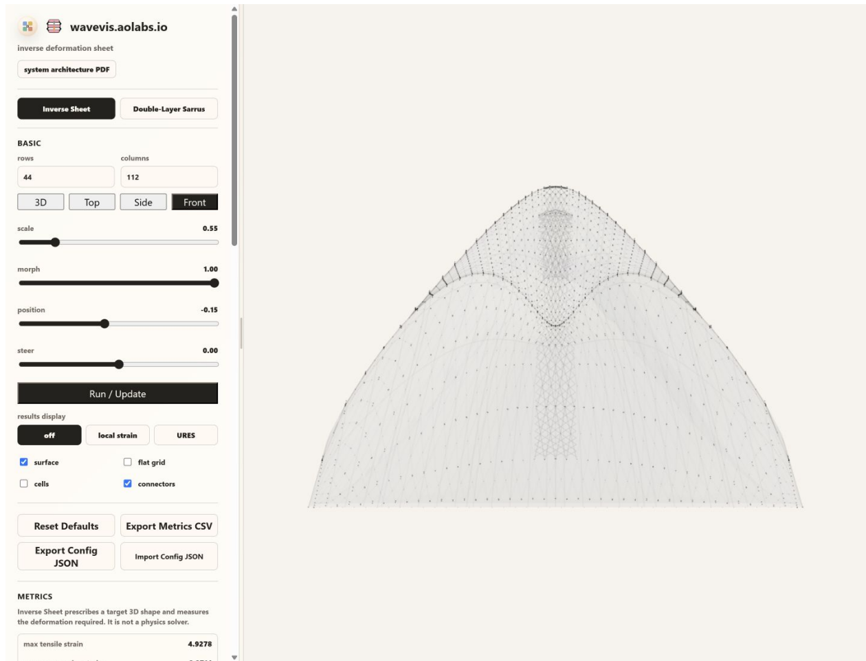
Figure 8. Candidate421 browser-rendered Front view for the same default state. This separate product camera compresses front depth, bounds the terminal lip contribution, depth-tests the pale grid against the lip, keeps rounded terminal width, and shows the center X-cell linkage through the projected cap rather than hiding mechanism state behind a pasted cap layer. The June 27 projection checkpoint remains open against the June 24 front reference.
