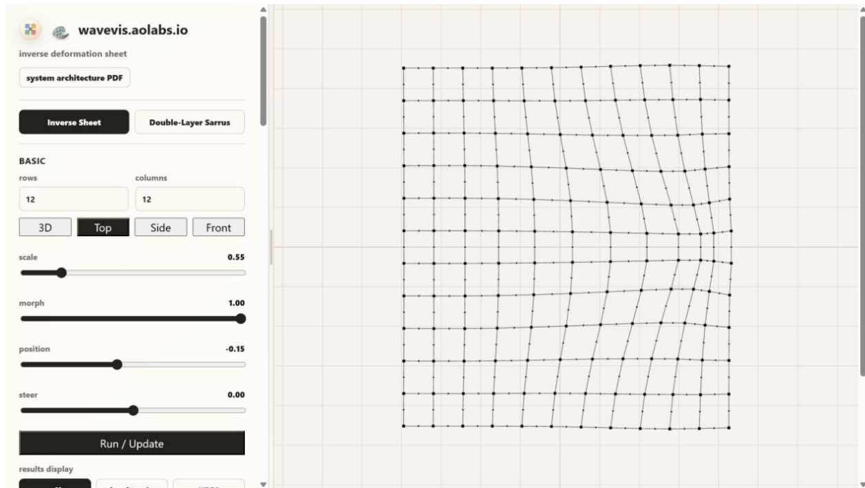
Figure 13. Candidate625 inspectable Top proof with rows=12, columns=12, surface=0, connectors=1, and cells=1. This low-density route exists so the hard cell contract can be inspected directly through the X legs and cells layers: a cell is not two nearby two-leg elements; it is one black square with four straight legs, and each visible connector is a spherical center-pair node used by exactly two neighboring cells.
