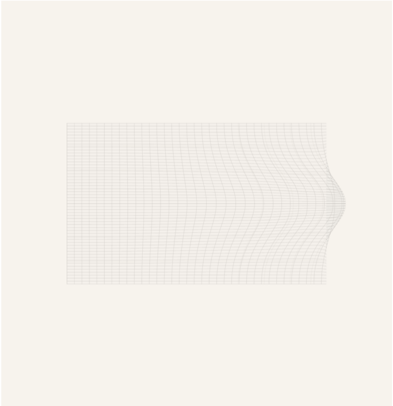
Figure 8. Current source-rendered Top view for the same default state. The surface-first view uses a continuous top-plan projection: the square sheet boundary remains visible while the interior grid now bends into a broader localized rounded footprint instead of the earlier narrow right-side band, rejected hard plateau, triangular fan, clipped patch, or oversized rectangular mechanism grid caused by reusing side-view framing.
