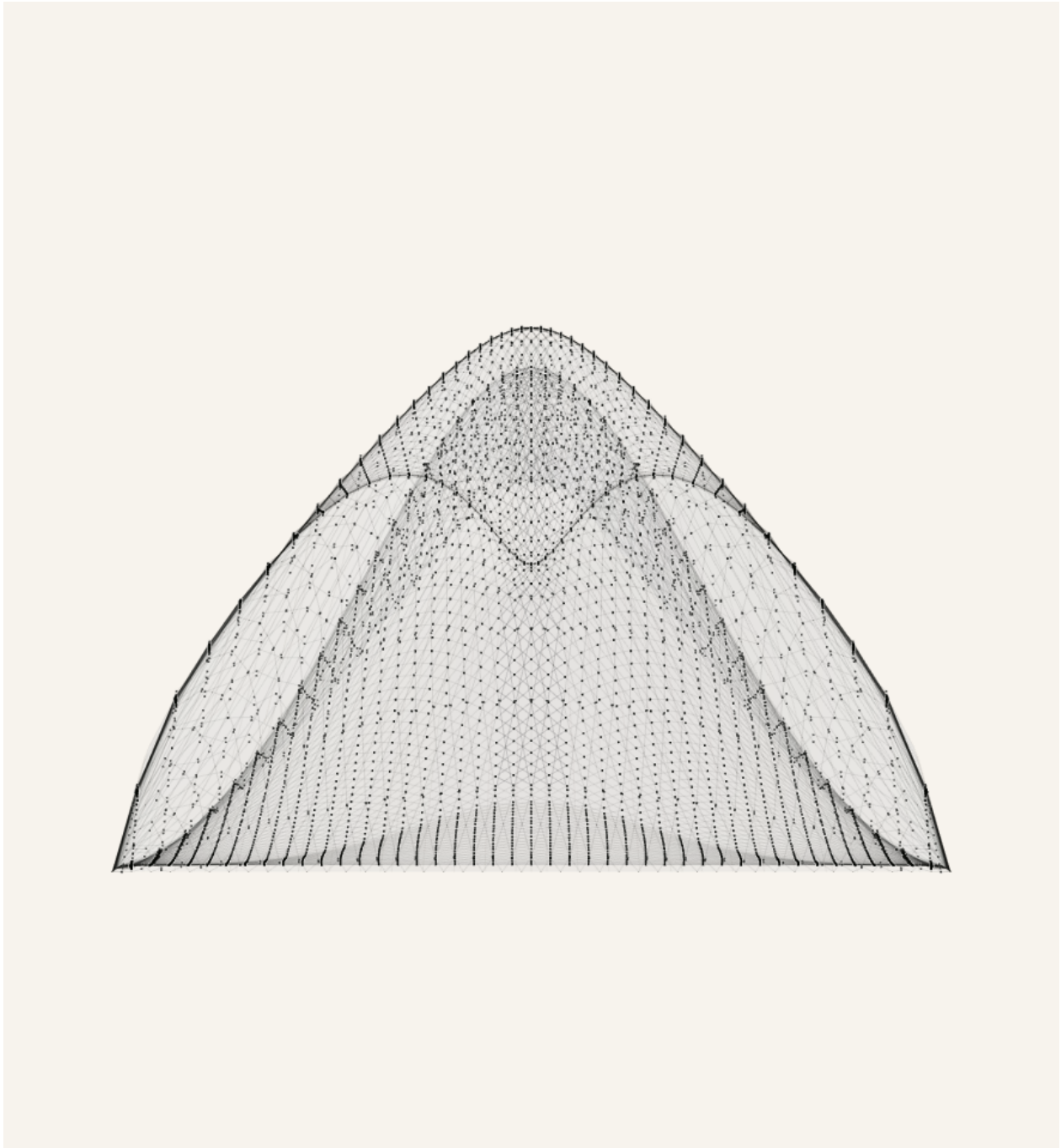
Figure 8. Candidate447 browser-rendered Front view for the same default state. This separate product camera compresses front depth, bounds the terminal lip contribution, depth-tests the pale grid against the lip, keeps rounded terminal width, and shows the center X-cell linkage through the projected cap rather than hiding mechanism state behind a pasted cap layer. The June 28 projection checkpoint remains open against the June 24 front reference.
