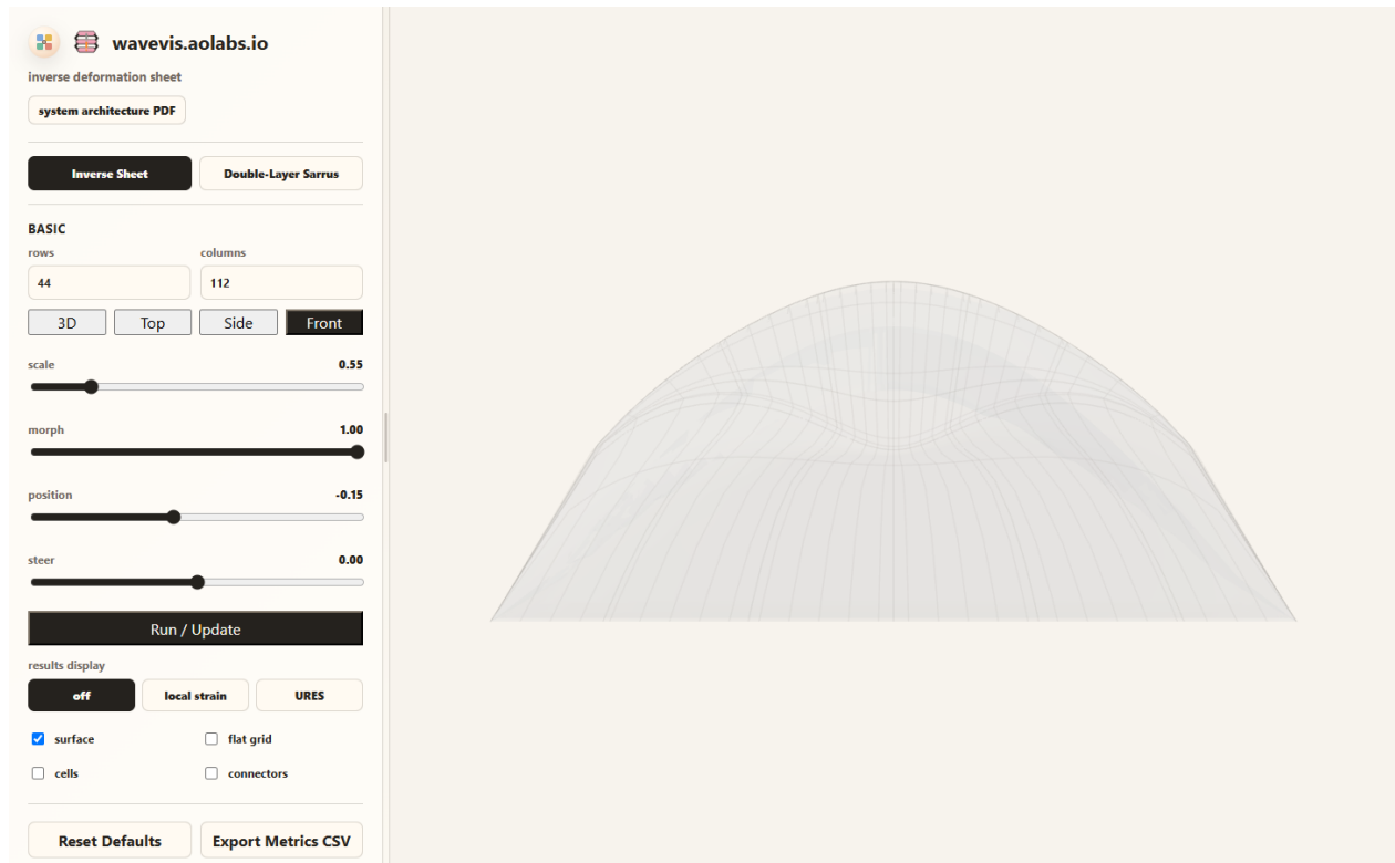
Figure 7. Current source-rendered Front view for the same default state. This separate product camera compresses front depth, bounds the terminal lip contribution, depth-tests the pale grid against the lip, keeps rounded terminal width, and uses a front-only pale lit surface cue plus a softened center-dipping underside on the same surface instead of the discarded pasted cap layer. It reduces the center-knot dimple and heavy construction trace, but remains open against the June 24 front reference.
