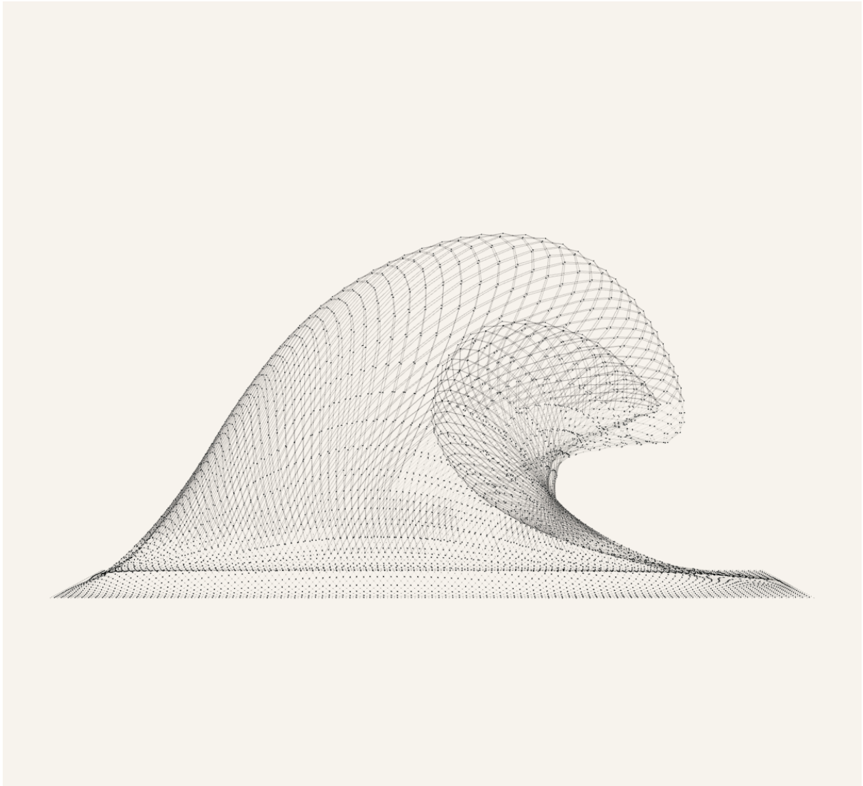
Figure 6. Candidate444 Side view with surface=0&connectors=1 . This X-only evidence removes the surface skin and shows the actual mechanism layer: each cell is a straight two-bar X, each diagonal is bisected at the center pivot, and neighboring cells meet at visible shared connector joints.
