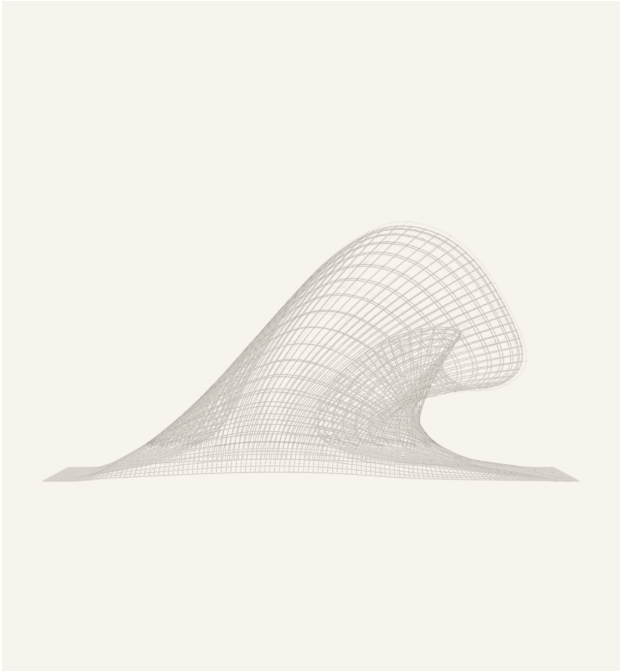
Figure 6. Candidate717 browser-rendered Side view for the default inverse-sheet state. The view keeps the readable surface subordinate to the actual mechanism: a lighter surface skin, pale side wire grid, soft grey one-center/four-leg cell bodies, spherical two-use connector nodes, and visible shared-joint rods are readable together without forming a black silhouette mass. The underside no longer contains the rejected bowl/dimple/cavity family, the perimeter border band is source-gated to stay flat, and Side uses a view-specific smoothed curled profile rather than the capped Candidate661 side path. The reference-wave match is still open: this checkpoint closes the surface-silhouette failure, but it remains sparse and approximate rather than a completed Moana-like plunge.
