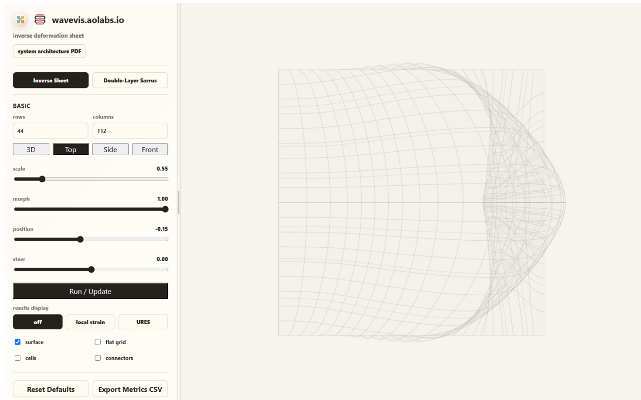
Figure 6. Current source-rendered Top view for the same default state. The smooth gridded surface is visible as one square reference sheet so the footprint can be checked directly. This is the gate that catches the June 22 failure: the plan footprint must read as a localized wave body on a square base, not as a large triangle, wedge, inset patch, or oversized rectangular mechanism grid caused by reusing side-view framing.
