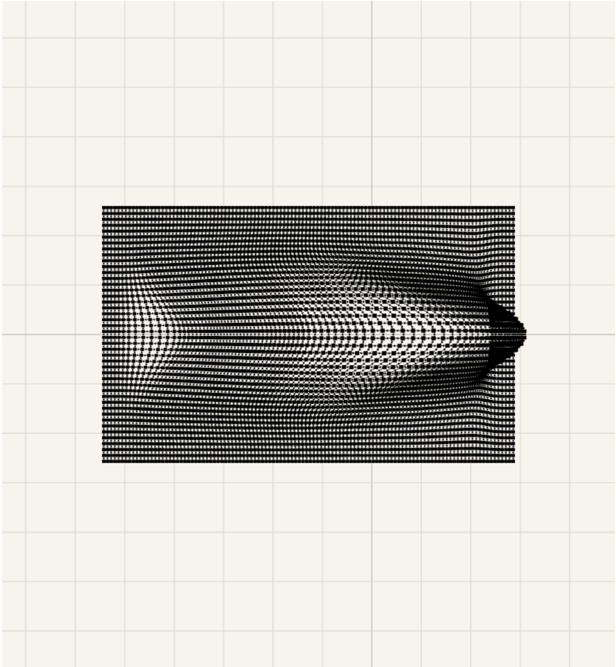
Figure 12. Candidate670 Top view with surface=0&connectors=1&cells=1 . This proof view is intentionally dense because it shows the whole array through the X legs and cells layers. Each visible black square cell is the body for four straight legs, each opposite pair remains collinear/equal through the center, and adjacent cells meet at spherical two-use connector nodes. This is the current hard mechanism acceptance test, not a decorative overlay.
