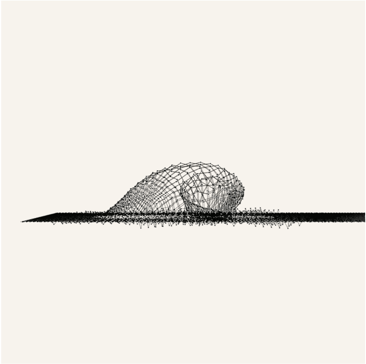
Figure 6. Candidate498 Side view with surface=0&connectors=1 . This X-only evidence removes the surface skin and shows the actual mechanism layer: each cell is a straight two-bar X, each diagonal is bisected at the center pivot, and neighboring cells meet at visible shared connector pins through real center-to-connector rods.
