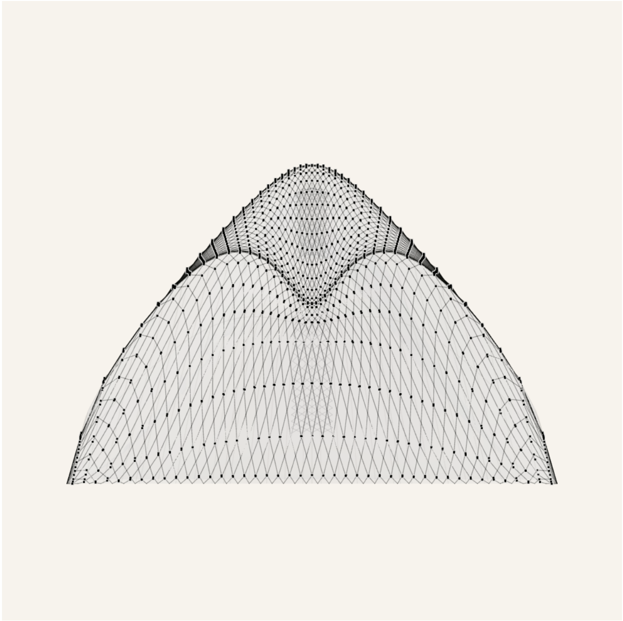
Figure 8. Candidate498 browser-rendered Front view for the same default state. This separate product camera compresses front depth, bounds the terminal lip contribution, depth-tests the pale grid against the lip, keeps rounded terminal width, and shows the center X-cell linkage through the projected cap rather than hiding mechanism state behind a pasted cap layer. The June 28 projection checkpoint remains open against the June 24 front reference.
