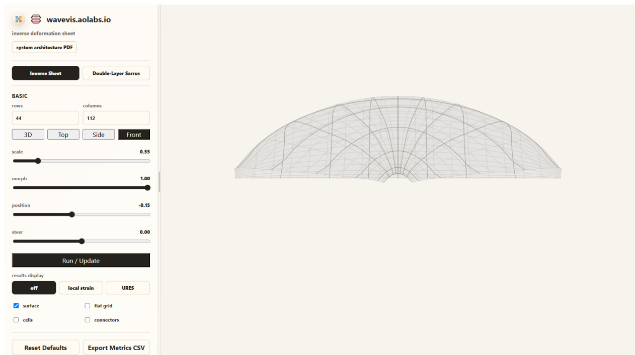
Figure 5. Current source-rendered Front view for the same default state. This view was added as a separate product camera so the spanwise mound and lip-cap read can be checked directly against the June 24 three-view reference.
