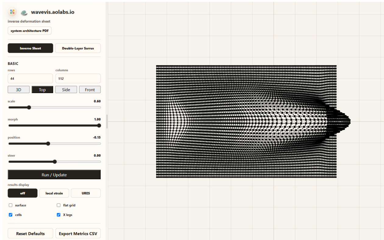
Figure 12. Candidate660 Top view with surface=0&connectors=1&cells=1. This proof view is intentionally dense because it shows the whole array through the X legs and cells layers. Each visible black square cell is the body for four straight legs, each opposite pair remains collinear/equal through the center, and adjacent cells meet at spherical two-use connector nodes. This is the current hard mechanism acceptance test, not a decorative overlay.
