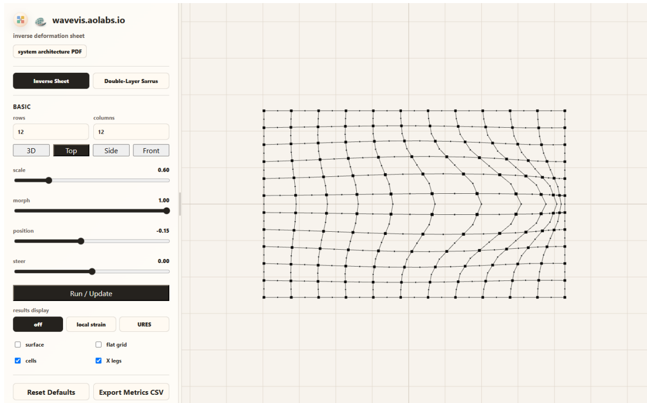
Figure 13. Candidate660 inspectable Top proof with rows=12, columns=12, surface=0, connectors=1, and cells=1. This low-density route exists so the hard cell contract can be inspected directly through the X legs and cells layers: a cell is not two nearby two-leg elements; it is one black square with four straight legs, opposite pairs are collinear and equal through the center, and each visible connector is a spherical node used by exactly two neighboring cells.
