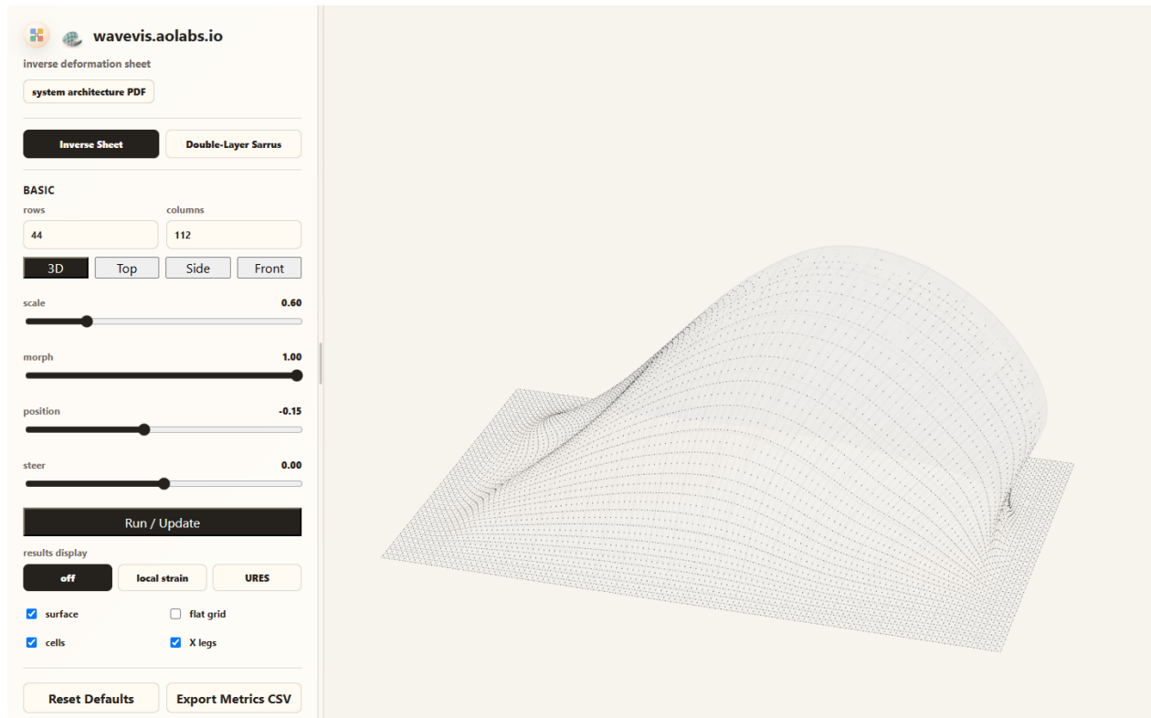
Figure 8. Candidate660 browser-rendered 3D/isometric view for the same default state. The default presentation retains the recovered geometry floor, restored isometric camera, source-profile readable surface skin, pale wire grid, black square four-leg X cells, spherical two-use connector nodes, and a much lighter surface-on proof overlay. The lighter overlay, no-cavity side gate, terminal taper gate, and perimeter-strip gate reduce the false dark throat/perimeter pocket without adding a fake bridge. This figure remains an improved open visual-match boundary rather than an exact reference match.
