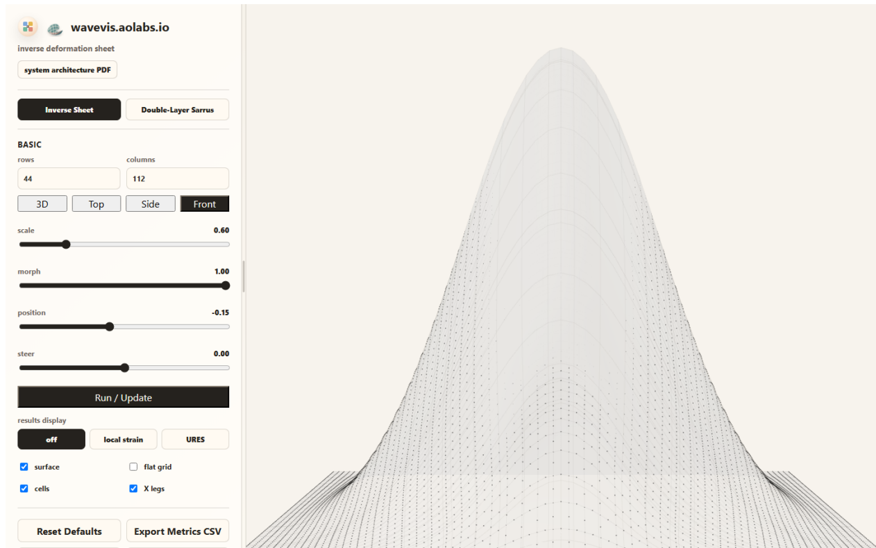
Figure 9. Candidate660 browser-rendered Front view retained as the separate spanwise product camera. This view compresses front depth, bounds the terminal lip contribution, depth-tests the pale grid against the lip, keeps rounded terminal width, and shows the black-square X-cell linkage with spherical connector nodes through the projected cap rather than hiding mechanism state behind a pasted cap layer. The projection checkpoint remains open against the June 24 and June 28 references.
