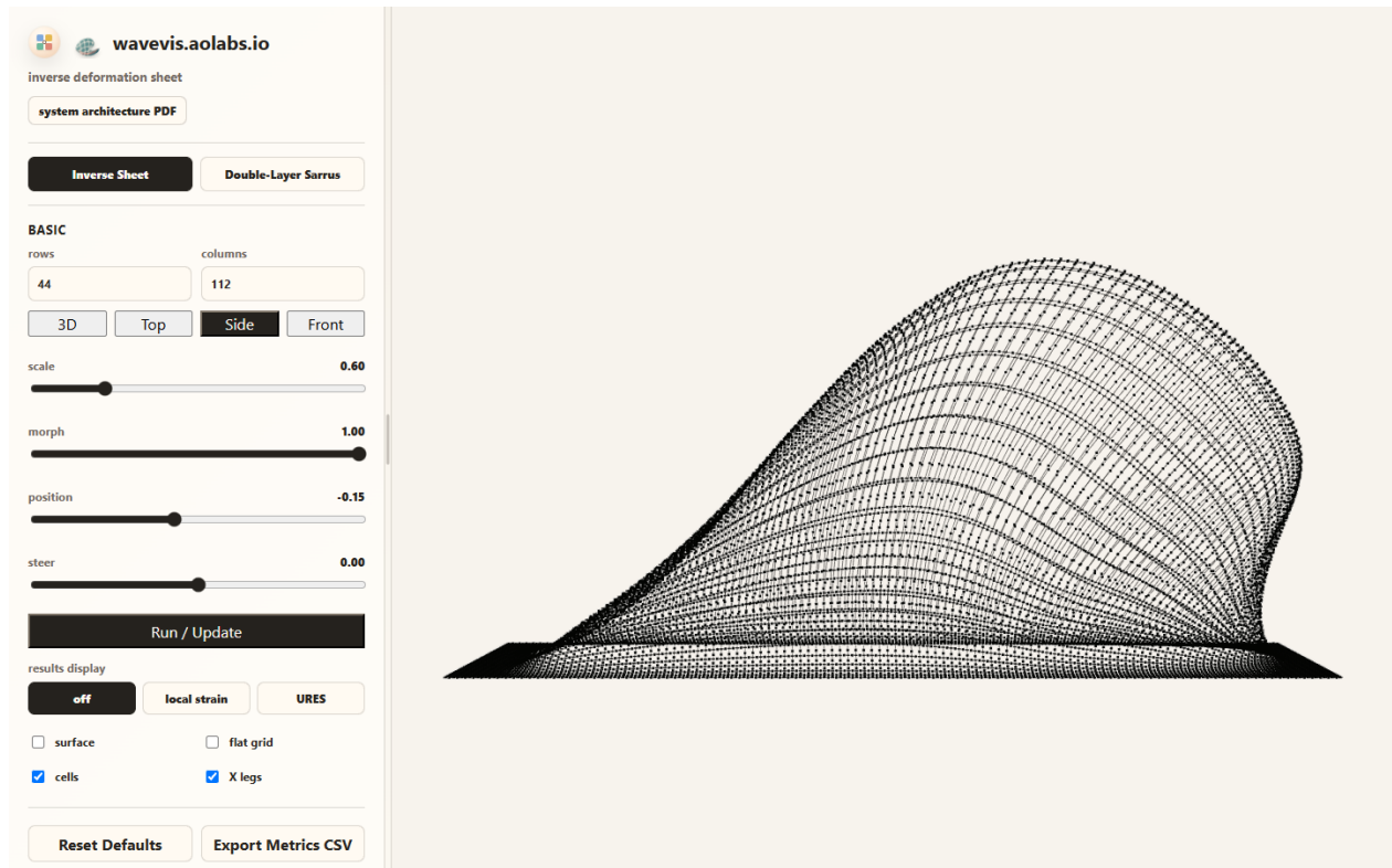
Figure 7. Candidate660 Side view with surface=0&connectors=1&cells=1 . This X-only evidence removes the surface skin and shows the actual mechanism layer: each cell is one black square with four straight center-to-connector legs, opposite pairs are equal length and collinear through the cell center, and every connector is a spherical physical node with exactly two attached leg uses. Neighboring cells meet through visible connector nodes; no between-cell connector is allowed to become an X or a four-cell joint.
