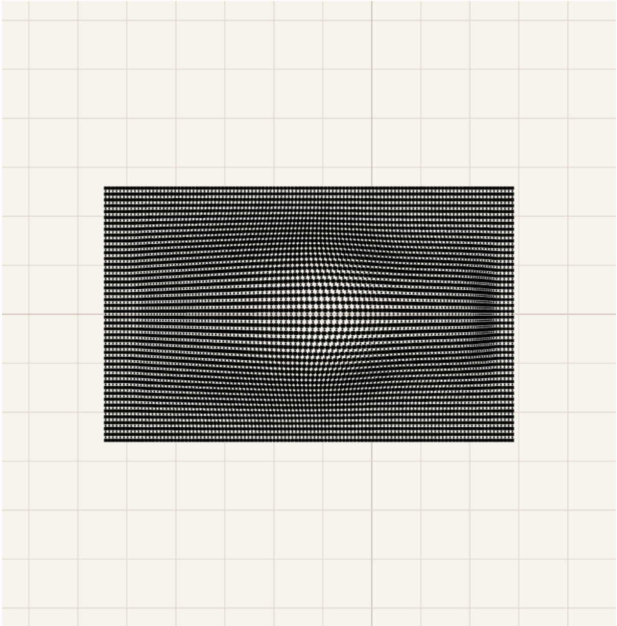
Figure 12. Candidate722 Top view with surface=0&connectors=1&cells=1 . This proof view is intentionally dense because it shows the whole array through the X legs and cells layers. Each visible black square cell is the body for four straight legs, each opposite pair remains collinear/equal through the center, and adjacent cells meet at spherical two-use connector nodes. This is the current hard mechanism acceptance test, not a decorative overlay.
