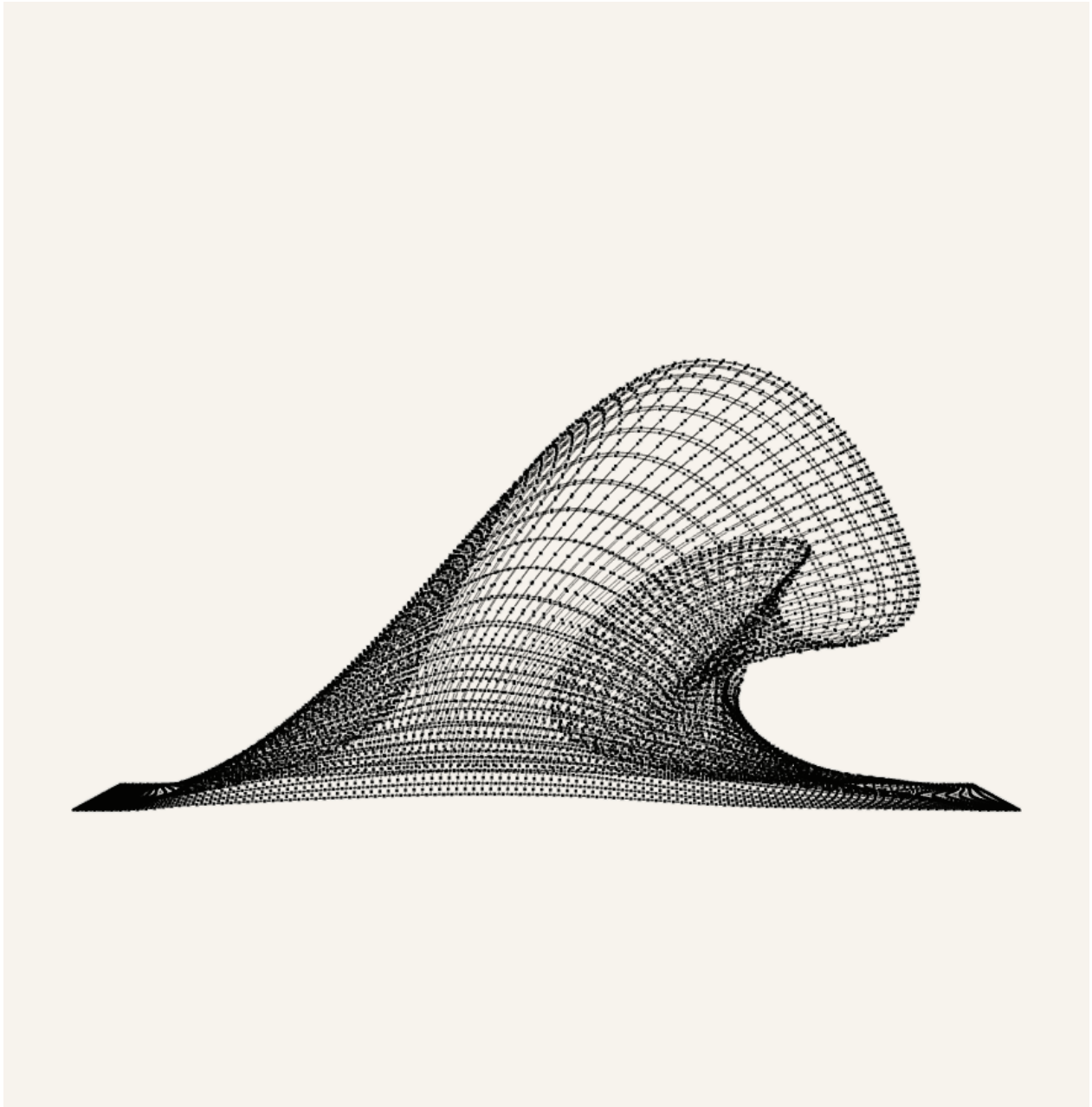
Figure 7. Candidate722 Side view with surface=0&connectors=1&cells=1 . This X-only evidence removes the surface skin and shows the actual mechanism layer after the side readable-profile split: each cell is one black square with four straight center-to-connector legs, opposite pairs are equal length and collinear through the cell center, and every connector is a spherical physical node with exactly two attached leg uses. Neighboring cells meet through visible connector nodes; no between-cell connector is allowed to become an X or a four-cell joint.
