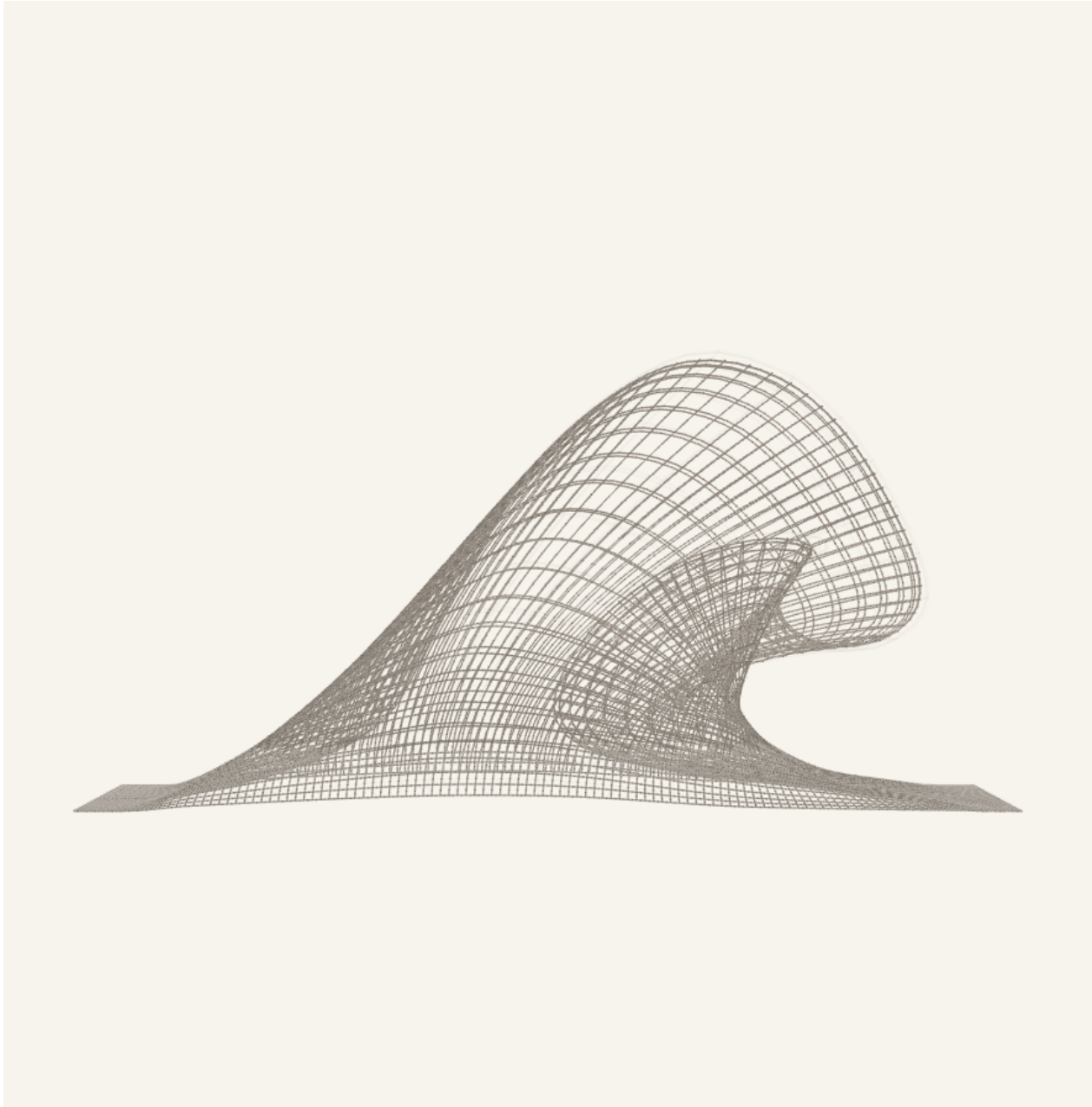
Figure 6. Candidate722 browser-rendered Side view for the default inverse-sheet state. The view keeps the readable surface subordinate to the actual mechanism: a lighter surface skin, stronger muted X-cell ink, one-center/four-leg cell bodies, spherical two-use connector nodes, and visible shared-joint rods are readable together without forming a black silhouette mass. Candidate722 routes the upper terminal throat frames into a softer mechanism layer and raises the normal product-view linkage contrast so the full sheet remains visible instead of reading as a surface shell. The underside no longer contains the rejected bowl/dimple/cavity family, the perimeter border band is source-gated to stay flat, and Side uses a view-specific smoothed curled profile rather than the capped Candidate661 side path. The reference-wave match is still open: this checkpoint closes the surface-silhouette failure and improves full-mechanism visibility, but it remains sparse and approximate rather than a completed Moana-like plunge.
