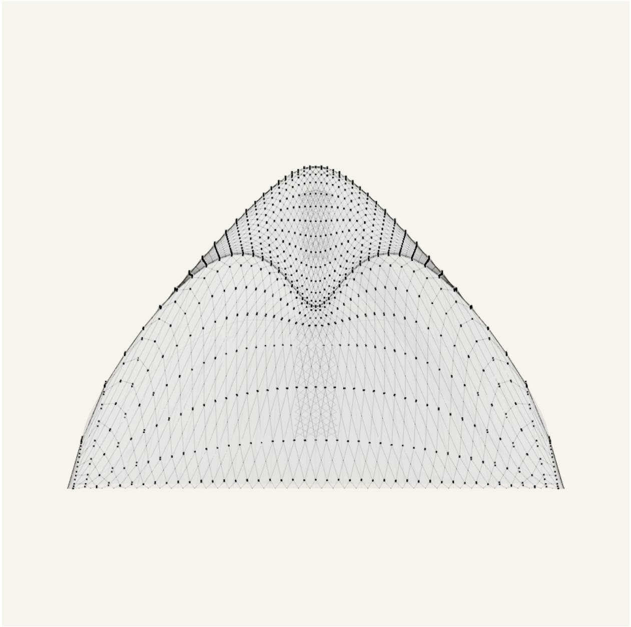
Figure 8. Candidate478 browser-rendered Front view for the same default state. This separate product camera compresses front depth, bounds the terminal lip contribution, depth-tests the pale grid against the lip, keeps rounded terminal width, and shows the center X-cell linkage through the projected cap rather than hiding mechanism state behind a pasted cap layer. The June 28 projection checkpoint remains open against the June 24 front reference.
