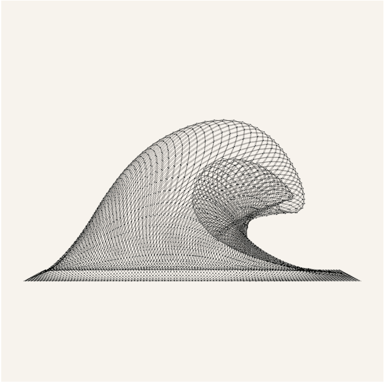
Figure 6. Candidate478 Side view with surface=0&connectors=1 . This X-only evidence removes the surface skin and shows the actual mechanism layer: each cell is a straight two-bar X, each diagonal is bisected at the center pivot, and neighboring cells meet at visible shared connector pins through real center-to-connector arms.
