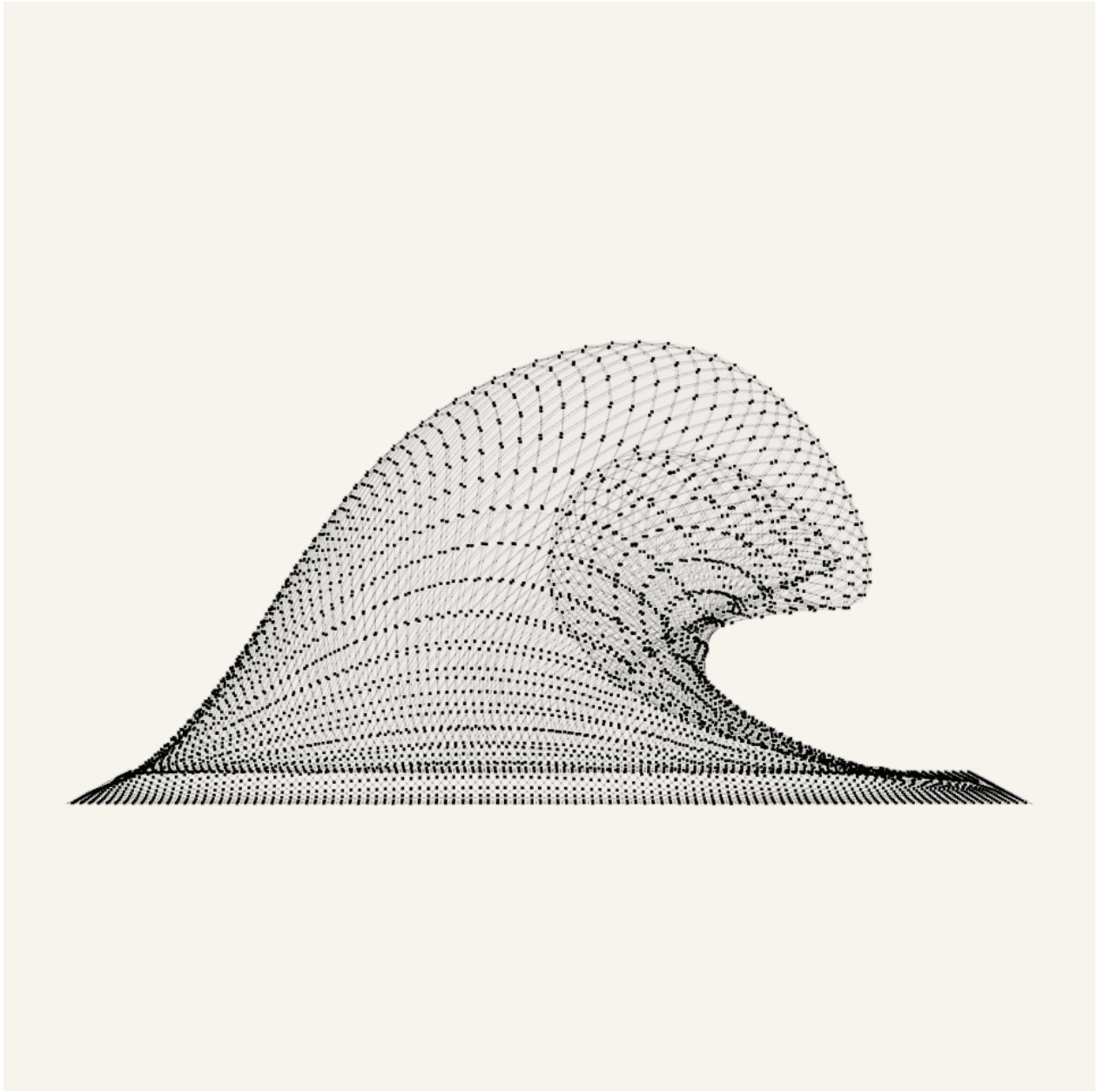
Figure 5. Candidate478 browser-rendered Side view for the default inverse-sheet state. The view is a full three-dimensional side camera with the readable surface, straight X-cell diagonals, center pivots, physical shared connector pins, and shared-joint arms visible together. It preserves the open exact-match boundary: the underside remains readable and the between-cell joints stay explicit, but the reference-wave match is still not closed.
