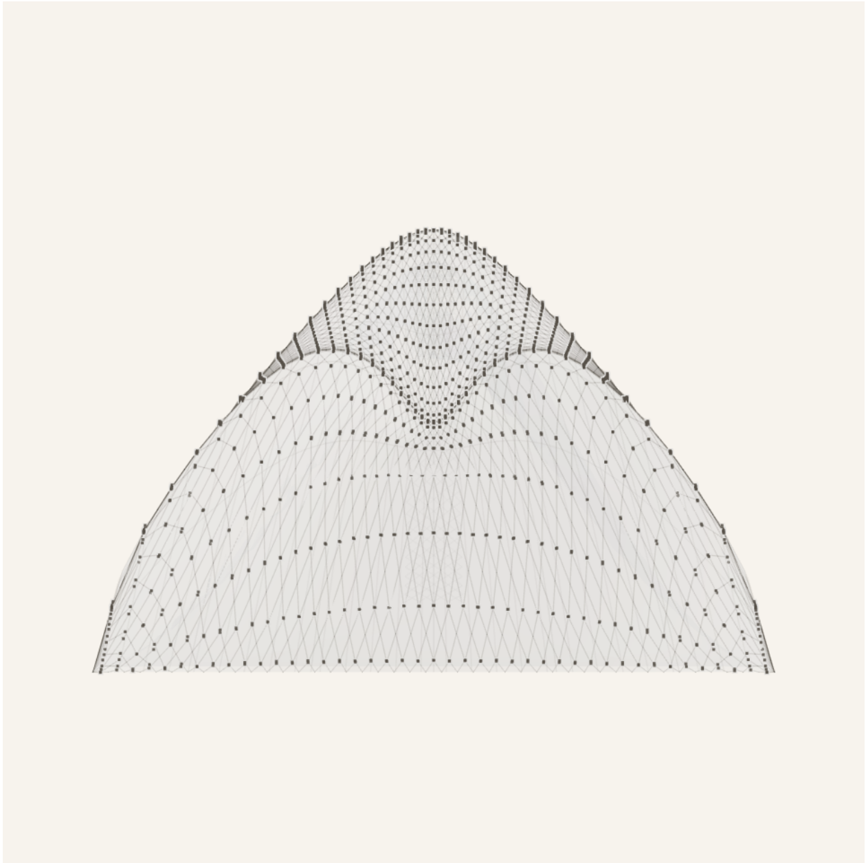
Figure 8. Candidate537 browser-rendered Front view for the same default state. This separate product camera compresses front depth, bounds the terminal lip contribution, depth-tests the pale grid against the lip, keeps rounded terminal width, and shows the center X-cell linkage through the projected cap rather than hiding mechanism state behind a pasted cap layer. The June 28 projection checkpoint remains open against the June 24 front reference.
