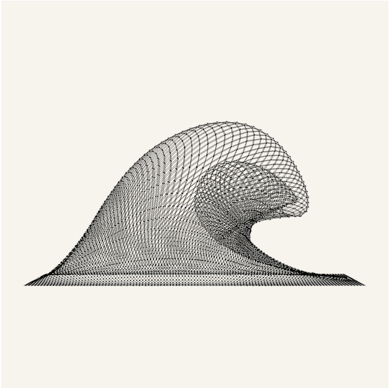
Figure 6. Candidate537 Side view with surface=0&connectors=1 . This X-only evidence removes the surface skin and shows the actual mechanism layer: each cell is a straight two-bar X, each diagonal is bisected at the center pivot, and neighboring cells meet at visible shared connector pins through real center-to-connector rods.
