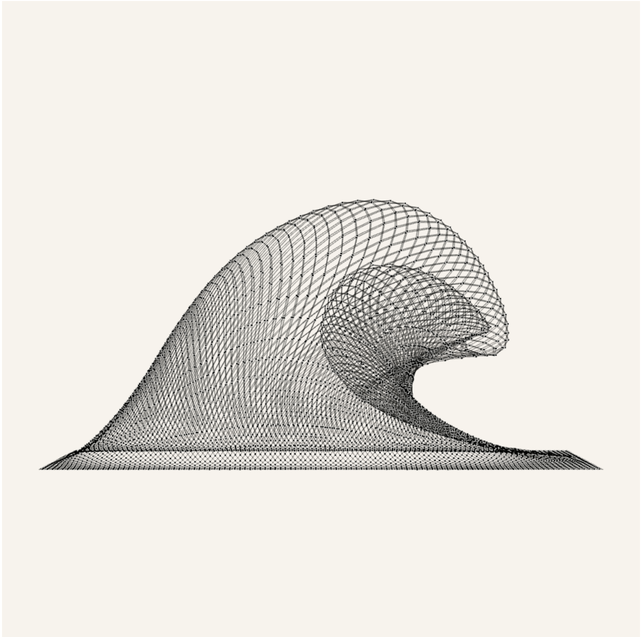
Figure 6. Candidate486 Side view with surface=0&connectors=1 . This X-only evidence removes the surface skin and shows the actual mechanism layer: each cell is a straight two-bar X, each diagonal is bisected at the center pivot, and neighboring cells meet at visible shared connector pins through real center-to-connector arms.
