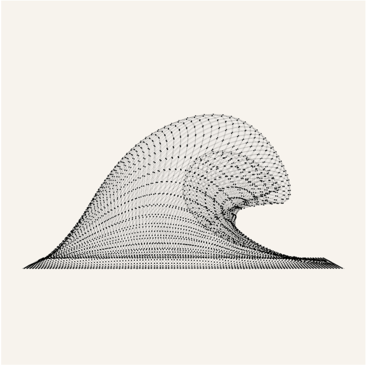
Figure 5. Candidate486 browser-rendered Side view for the default inverse-sheet state. The view is a full three-dimensional side camera with the readable surface, straight X-cell diagonals, center pivots, physical shared connector pins, and shared-joint arms visible together. It preserves the open exact-match boundary: the underside remains readable and the between-cell joints stay explicit, but the reference-wave match is still not closed.
