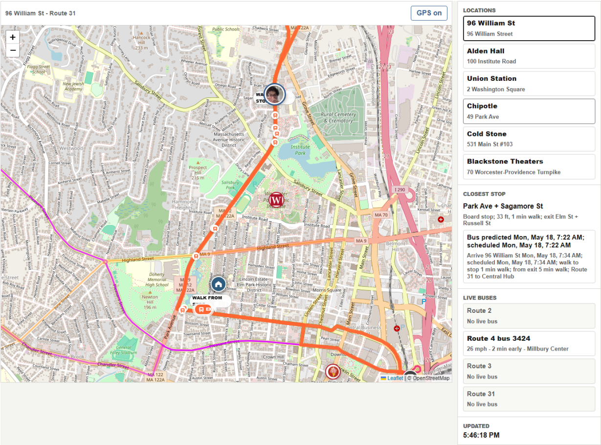
Figure 1. Stable live interface for selected WRTA destinations. The public app keeps saved destinations, route geometry, bus-stop symbols, live-bus state, and current-location state on one map while the side panel keeps boarding-stop and arrival rows in the same view. In this capture, simulated browser geolocation near Park Avenue and Sagamore Road selects Park Ave + Sagamore St as the boarding stop for a trip to 96 William Street, while Elm St + Russell St remains the exit-side stop. The timing row separates WRTA-derived bus arrival at the boarding stop from the derived destination-arrival estimate.
