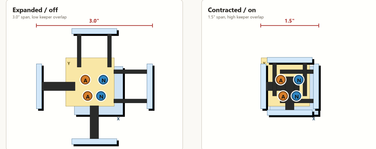
Figure 4. Opened two-layer magnetic state schematic. Both panels show the X and Y layers together. Orange rods mark Alnico; blue rods mark NdFeB. The expanded/off state shows the 3.0 inch span and low keeper overlap; the contracted/on state shows the 1.5 inch span and deeper overlap. The fork prongs end flush at the carrier-bar face.
