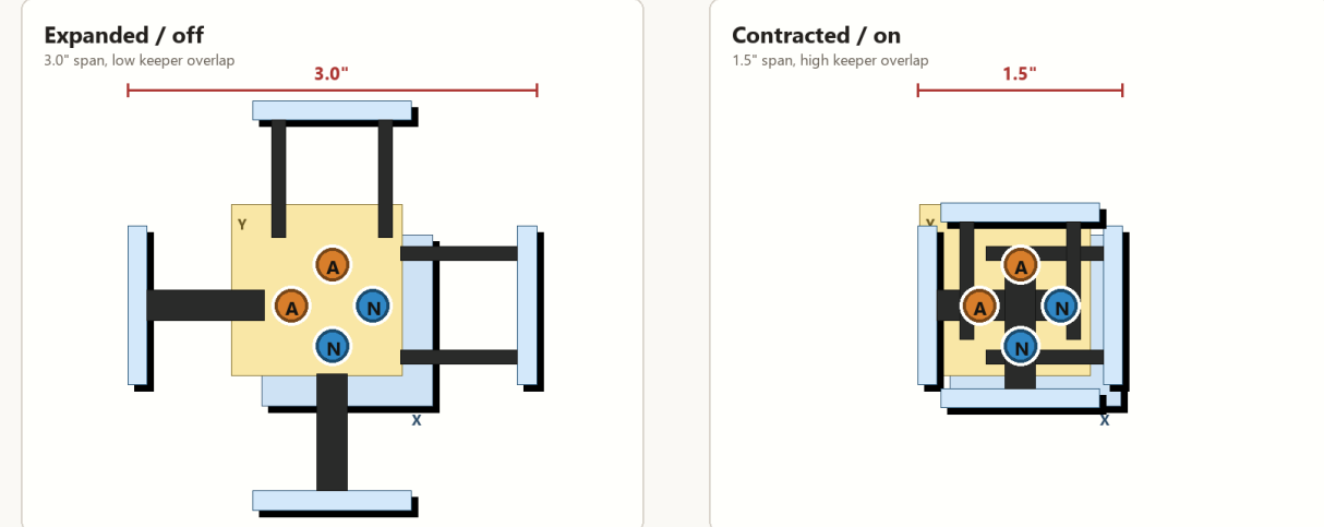
Figure 4. Opened two-layer magnetic state schematic. Both panels show the X and Y layers together. Orange rods mark Alnico; blue rods mark NdFeB. The Y-layer A/N pair is left-right, and the rotated X-layer A/N pair is top-bottom. The expanded/off state shows the 3.0 inch span and low keeper overlap; the contracted/on state shows the 1.5 inch span and deeper overlap. The fork prongs end flush at the carrier-bar face.
