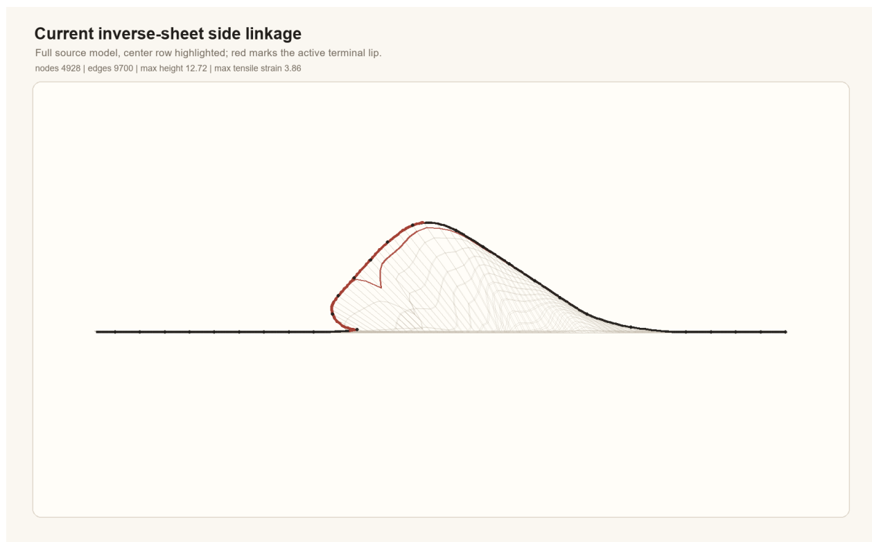
Figure 2. Current source-rendered side linkage for the default inverse-sheet state. This is not a cross-section. The full linkage sheet remains visible, and the side camera faces the rounded open throat, visible low return branch, and flat return in the same direction as the reference family.
