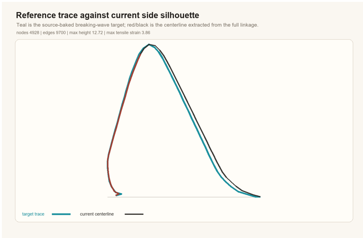
Figure 3. Current centerline silhouette against the normalized source-baked breaking-wave target. The overlay is the human-facing shape gate for this repair: it shows crest alignment, a smooth downturned terminal branch, and no closed angular interior loop while keeping the remaining reference difference explicit.
