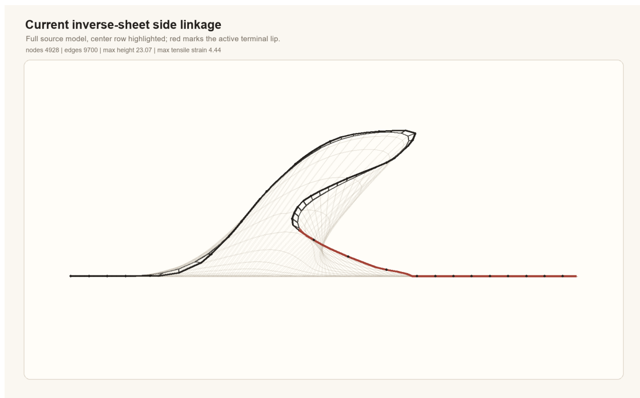
Figure 2. Current source-rendered side linkage for the default inverse-sheet state. This is not a cross-section. The full linkage sheet remains visible, the previous closed under-lip pocket is removed, and the terminal lip now tucks leftward from the shoulder while leaving an open throat before the flat return.
