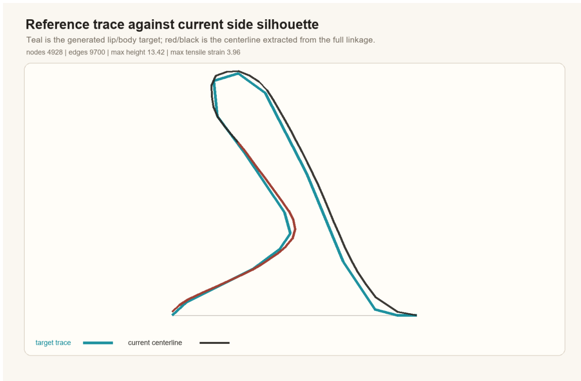
Figure 3. Current centerline silhouette against the normalized generated lip/body target. The overlay is the human-facing shape gate for this repair: it shows the crest alignment, lower inner return, and open throat while keeping the remaining reference difference explicit.
