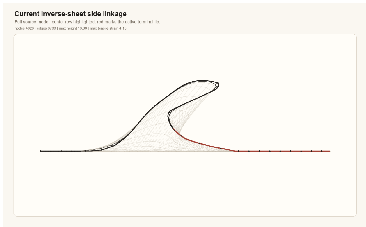
Figure 2. Current source-rendered side linkage for the default inverse-sheet state. This is not a cross-section. The full linkage sheet remains visible, the previous pointed sail and K-shaped return are removed, and the terminal lip now forms a rounded open throat before the flat return.
