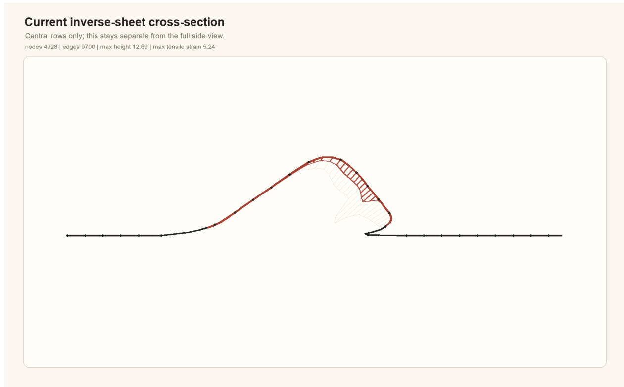
Figure 5. Current source-rendered cross-section for the same default state. This mode intentionally isolates central rows. It is useful for debugging the curl, but it is not allowed to substitute for the full 3D side view or 3D view.
