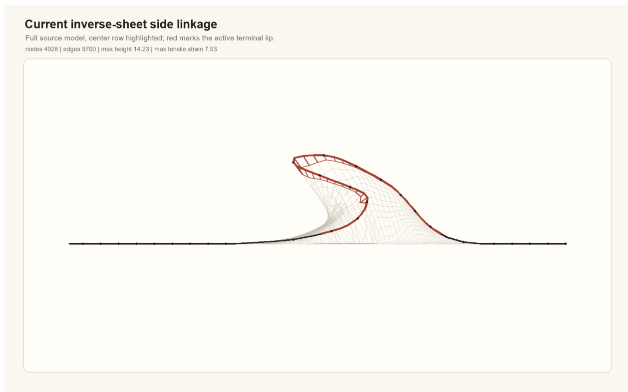
Figure 2. Current source-rendered side linkage for the default inverse-sheet state. This is not a cross-section. The full linkage sheet remains visible, and the side camera faces the rounded open throat and flat return in the same direction as the reference family.
