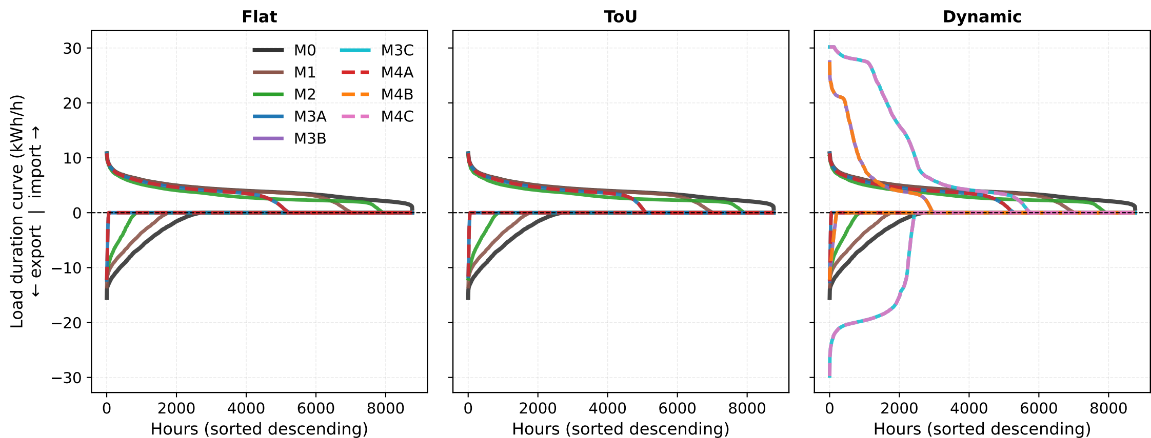
A: Behind-the-meter only (no market access)
