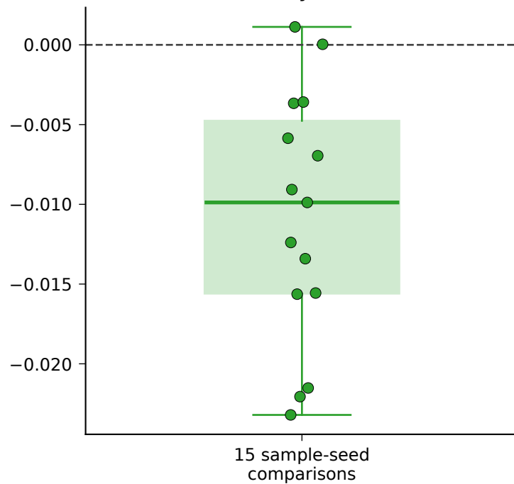
Activity delta
