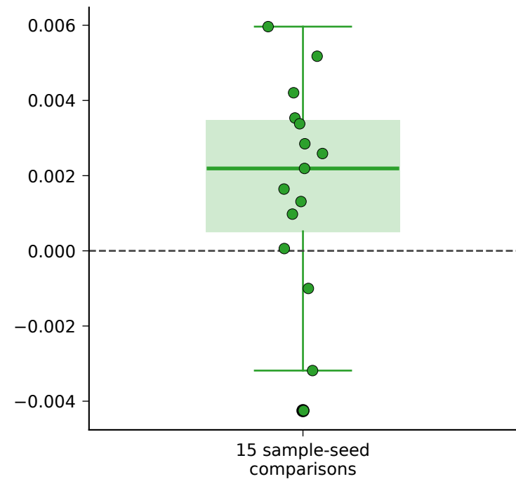
Loss delta
