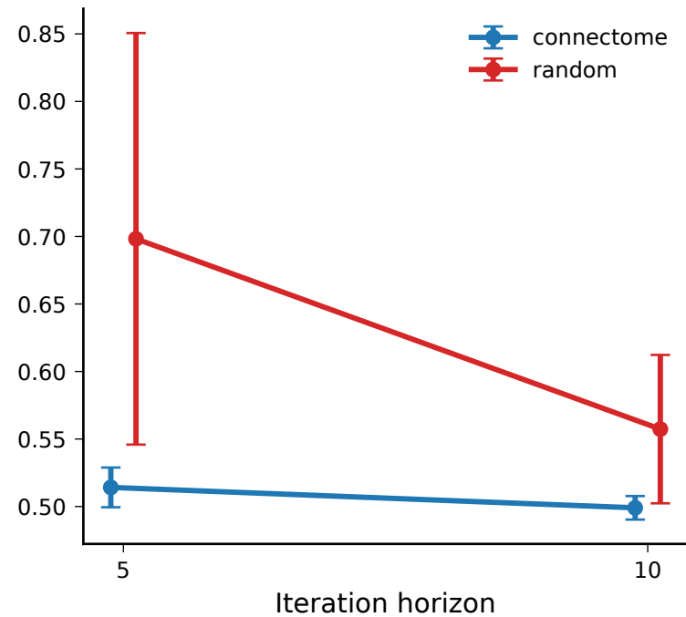
Task loss
