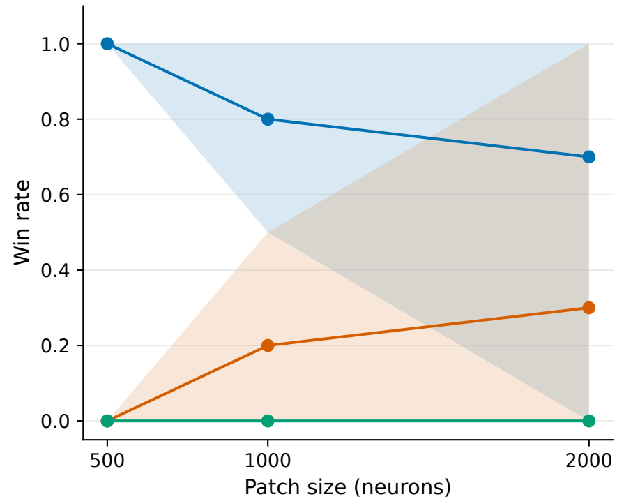
Scale robustness: win rate
