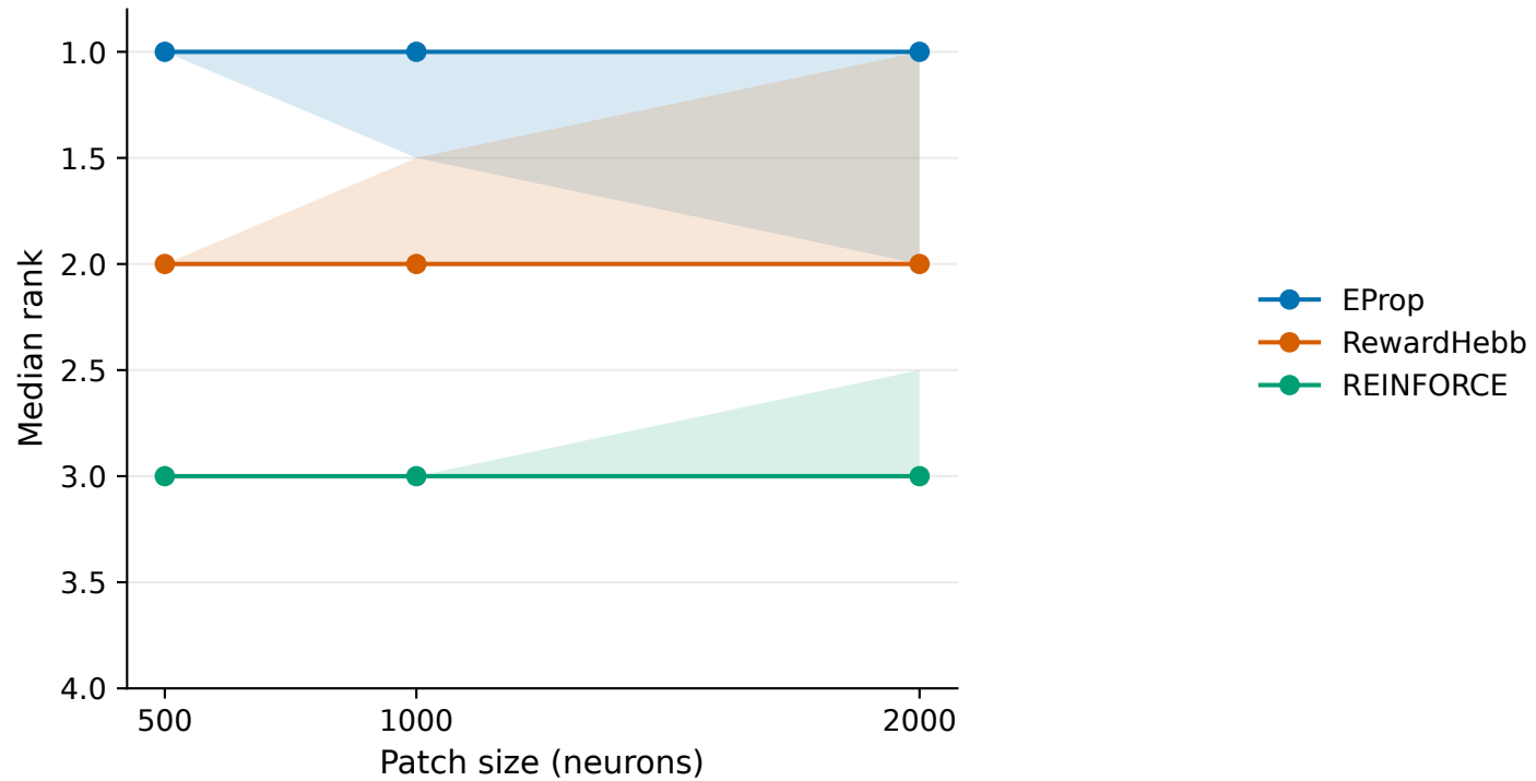
Scale robustness: rank
