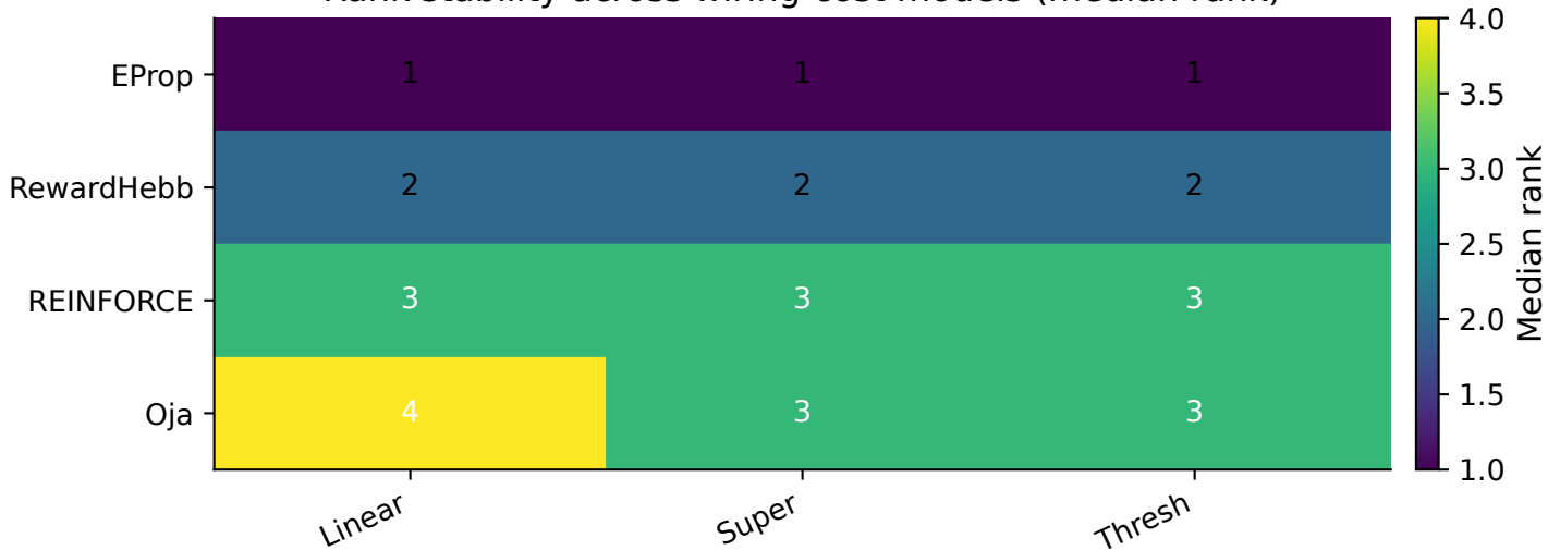
Rank stability across wiring-cost models (median rank)
