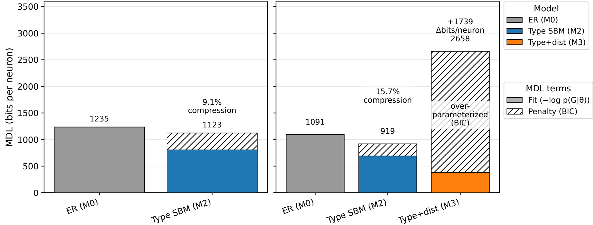
Model selection by MDL
