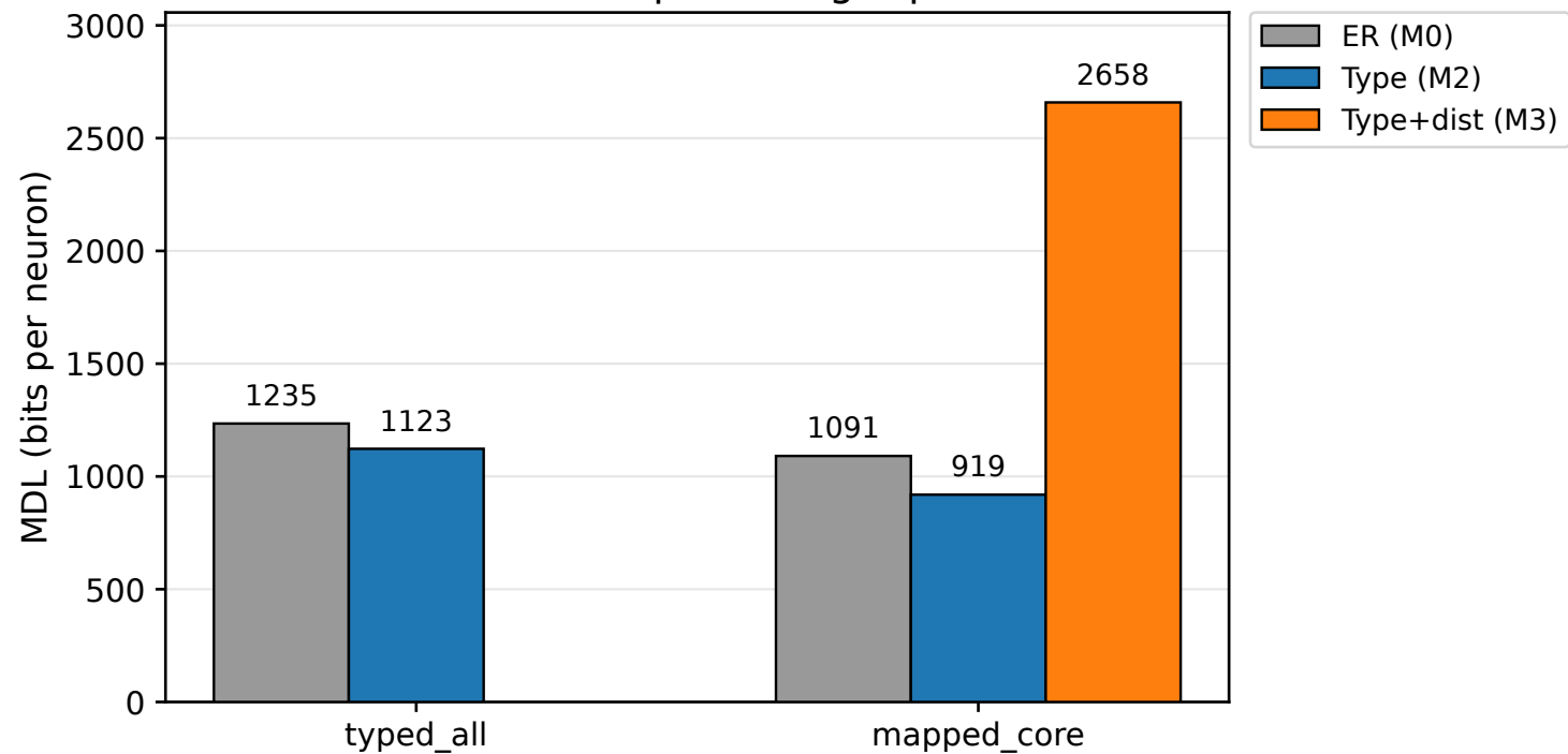
Connectome description length per neuron
